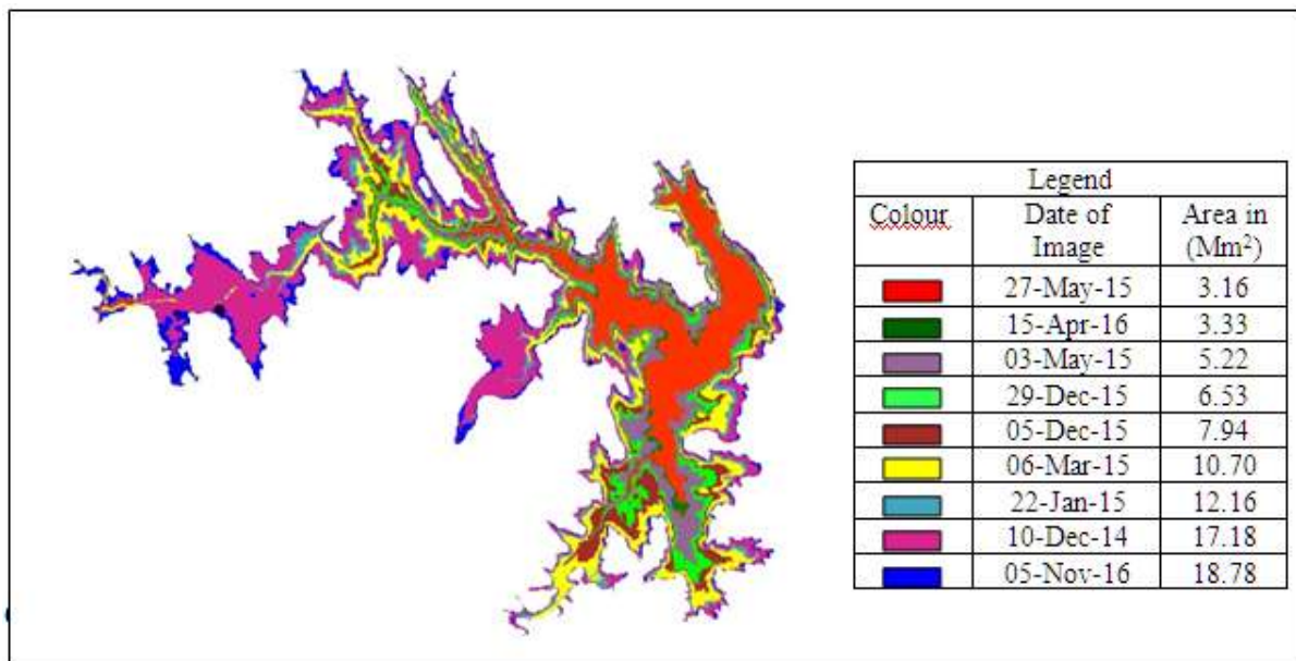
Fig. 4 : Water Spread Area for all satellite images
