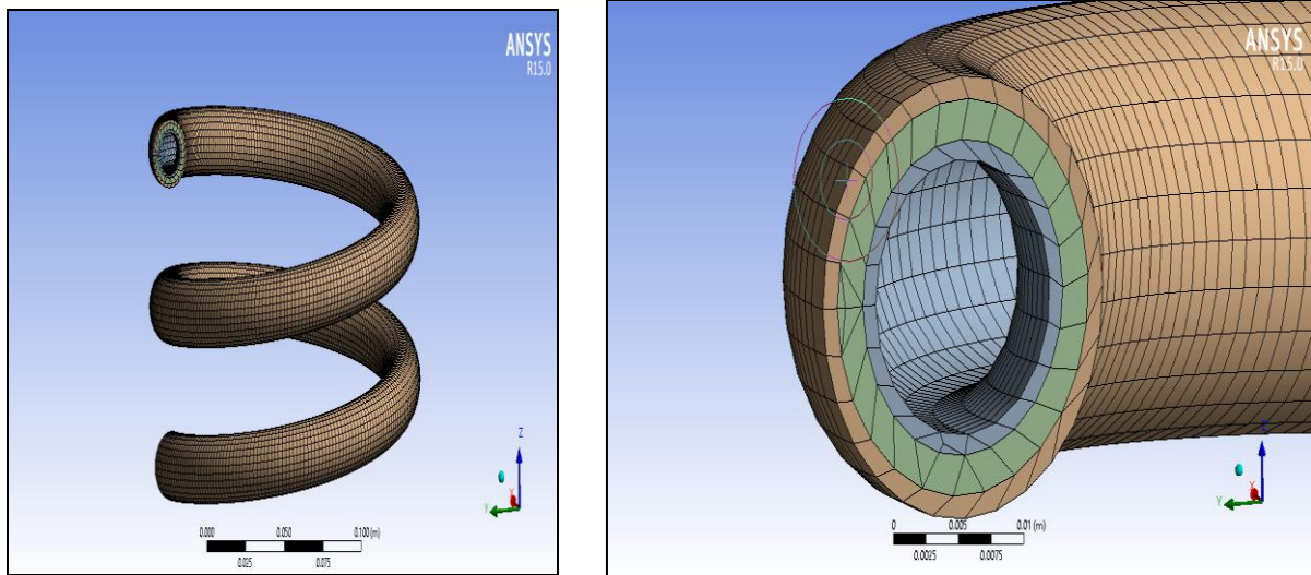
Figure 2. Meshing Structure of Helical Coil Tube
