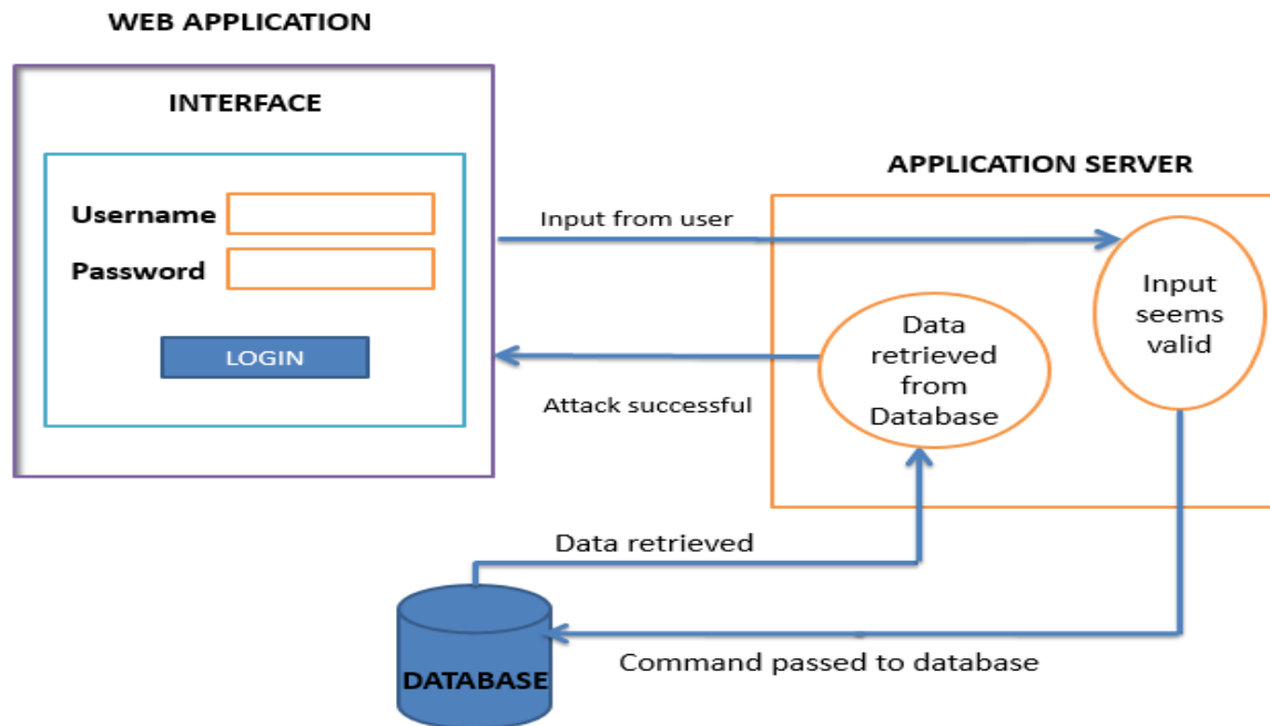
Figure 1: Attack performed on a web application's database
