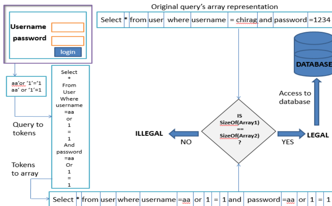
Figure 4: Query splitting process
