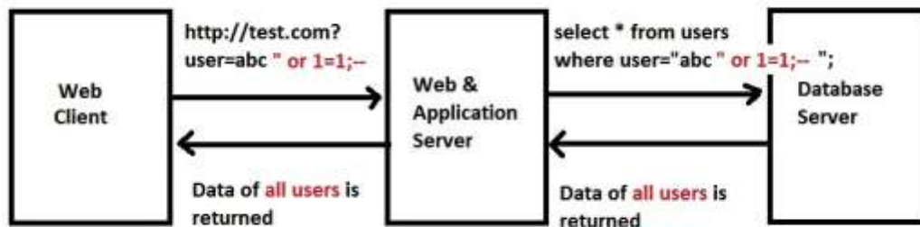
Figure 2: Malicious user input on the log in form
