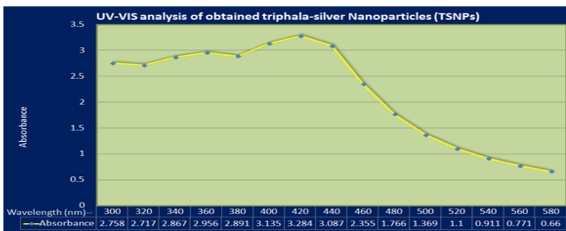
Figure 3: UV-VIS analysis of obtained triphala-silver Nanoparticles (TSNPs)
