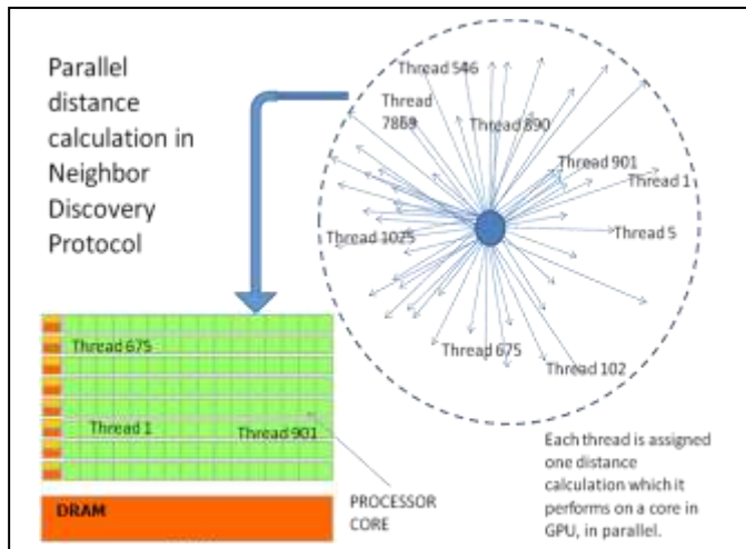
Figure 3: Distance calculations in NDP on a CPU-GPU system will have higher parallelism opportunity
