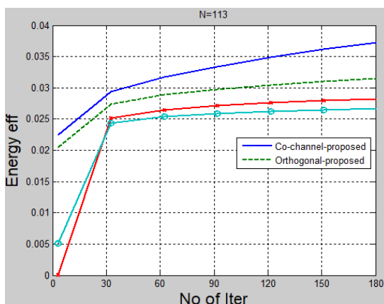
Fig.18: Energy efficiency at N=113 for proposed and base paper[18] technique.
