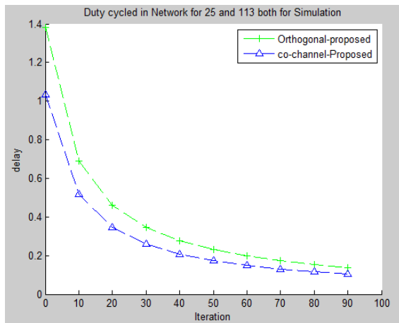
Fig. 8: Duty cycle in Network for 25 and 113 for delay Fig. 9: No of active s-BS at N=25
