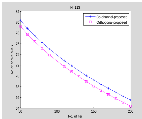
Fig. 10: No of active BS at N=113
