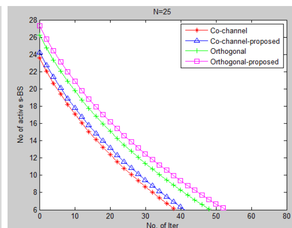
Fig. 12: No of Served UE at N=113 Fig. 13: No of active s-BS at N=25 for proposed and base paper[18] technique.
