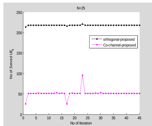
Fig. 11: No of Served UE at N=25
