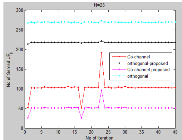
Fig. 15: No of Served UE at N=25 for proposed and base paper[18] technique.
