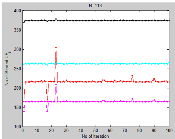
Fig. 16: No of Served UE at N=113 for proposed and base paper[18] technique.
