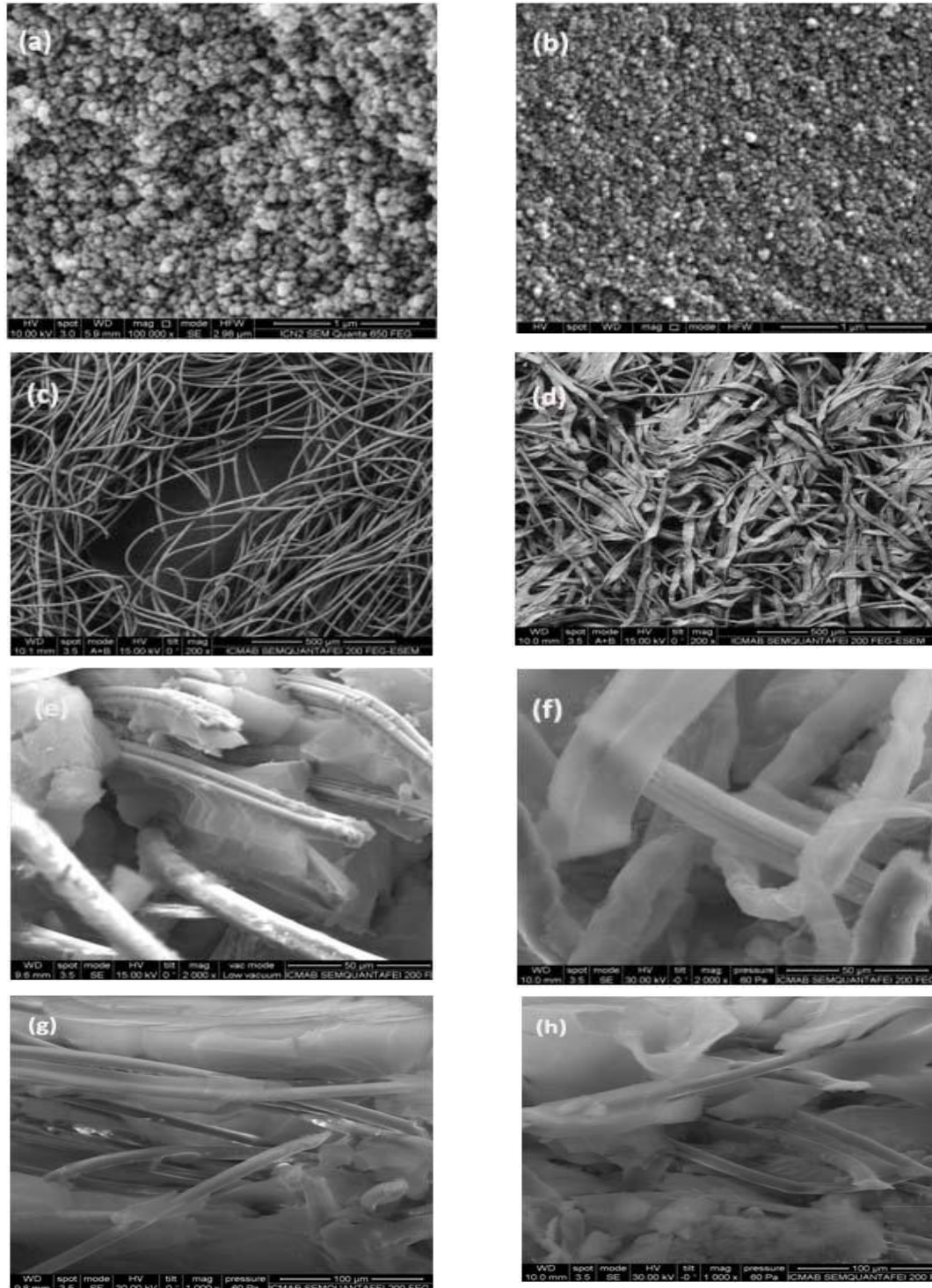
Fig (2). Scanning Electron Microscopy (SEM) micrographs of silica films: (a) Aerogel SiO 2 film (mag:100000X), (b) Cryogel SiO 2 film (mag:100000X), (c) Untreated gauze (mag: 200X), (d) Untreated non-woven (mag:200X), (e) Aerogel SiO 2 film on gauze (mag: 2000X), (f) Aerogel SiO 2 film on non-woven (mag:2000X), (g) Cryogel SiO 2 film on gauze (mag:1000X) and (h) Cryogel SiO 2 film on non-woven (mag:1000X).
