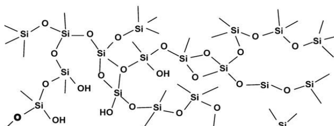
Fig (4). The silicon dioxide skeleton for aerogel and cryogel samples
