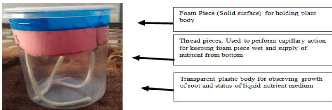
Fig. 3 Final structure of hydroponical system: Indoor use (home and office)
