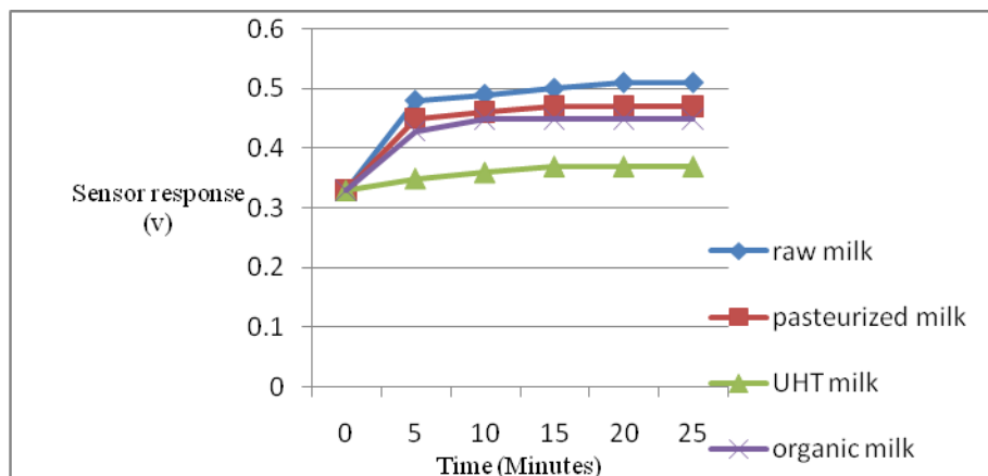
Fig.4: Variation of acetic acid in different types of milk shows the distinction of raw milk, pasteurized milk, UHT and organic milk.
