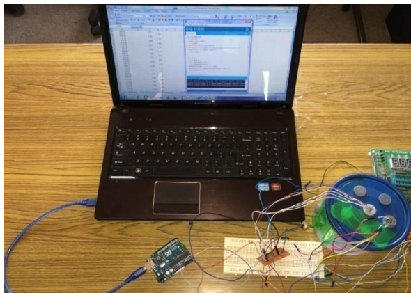
Fig. 2: Experimental setup of prototype of electronics nose
