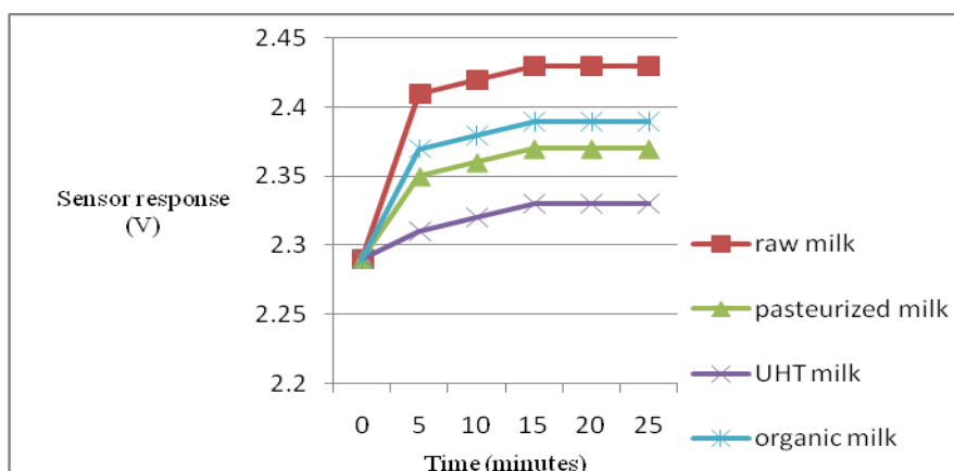
Fig. 5: Variation of Carbon dioxide in different types of milk shows the distinction of raw milk, pasteurized milk, UHT and organic milk
