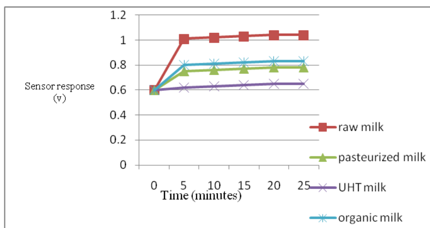
Fig. 3: Variation of acetaldehyde in different types of milk shows the distinction of raw milk, pasteurized milk, UHT and organic milk.
