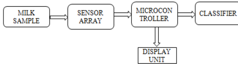
Fig.1: Block diagram of the Prototype Electronic nose
