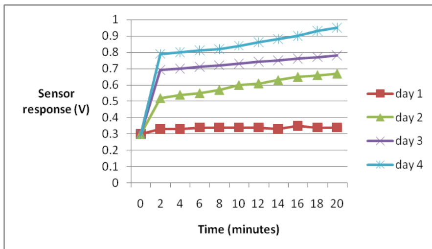
Fig. 7: Shows the aging of the raw milk by the Variation of acetic acid in raw milk for different days(TGS 813).
