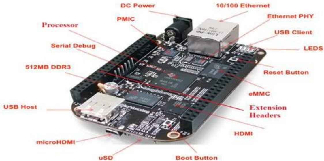
Fig. 3: Beaglebone Black Board-Components [ImgSrc: www.beagleboard.org]
