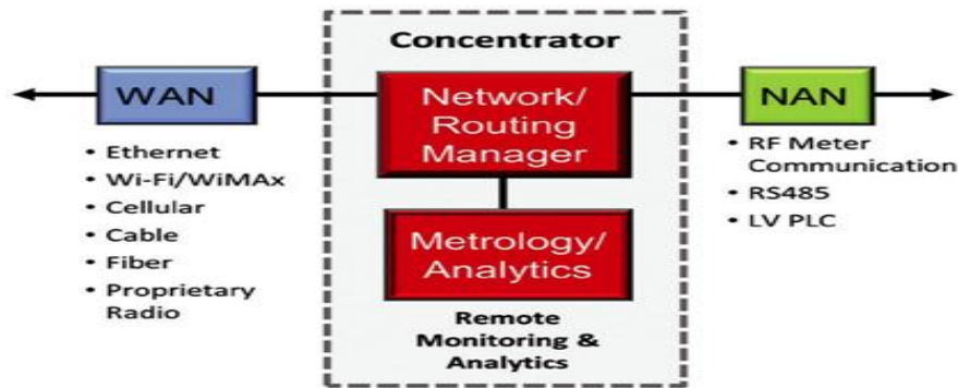
Fig 1: Data concentrator functional block diagram
