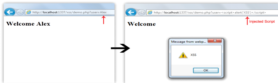
Figure 1: XSS Vulnerable Web Page before and after.
