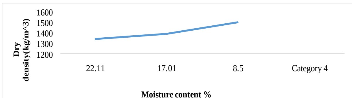
Fig 3: Variation of Moisture Content with Dry Density
