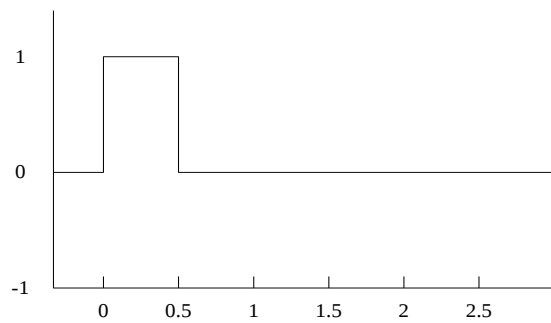
Fig.3: Haar scaling function \phi(2t) .
