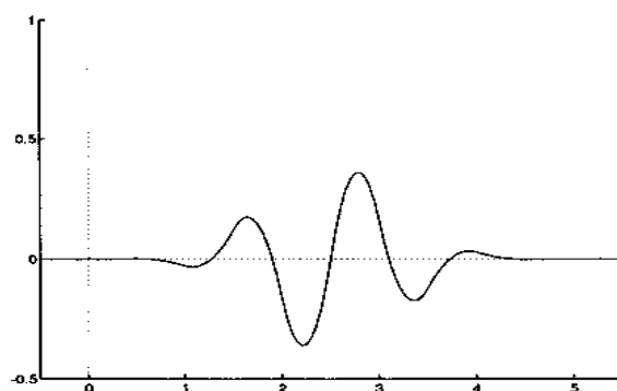
Fig. 9 Quadratic B Spline wavelet \psi_3(x)
