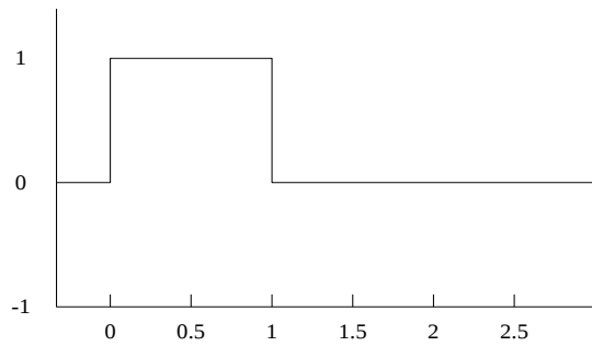
Fig.1: Haar scaling function \phi(t) .
