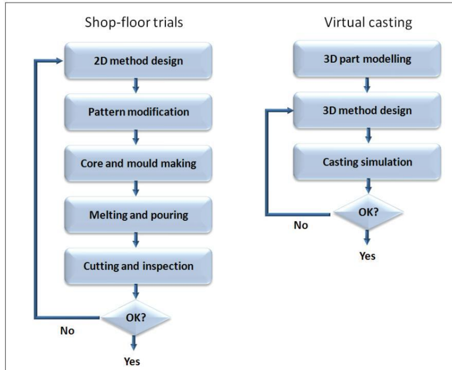
Fig.1 Actual and virtual casting process [1]
