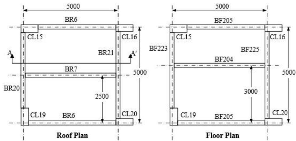
Fig 3.1: Roof and Floor Plan Of Model
