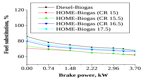
Fig.4.Variation of fuel substitution with brake power
