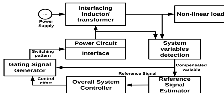
Figure 2 Active Power Filter Design
