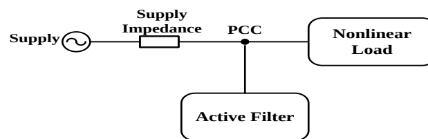
Figure 4 Shunt Active Power Filters
