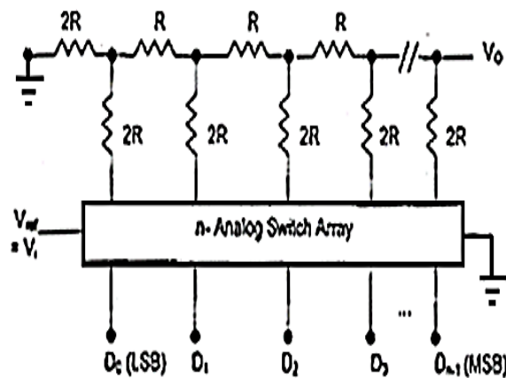
Fig. (2) n-bit R-2R Ladder Network
