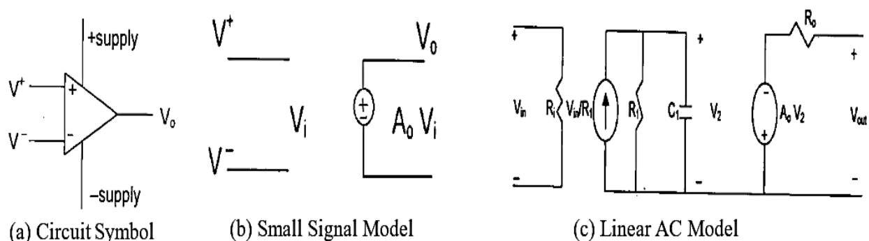
Fig. (1) Operational Amplifier (Op-Amp)
