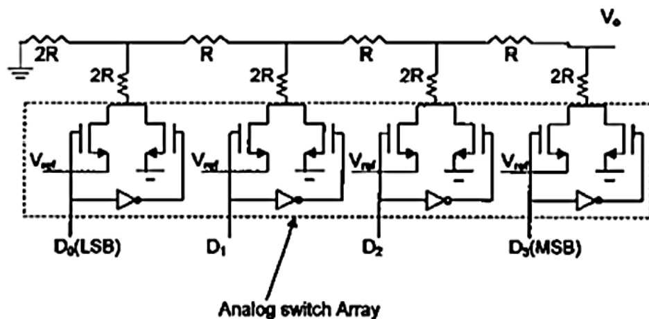
Fig. (5) R-2R Ladder Network driven by Digital Control Word
