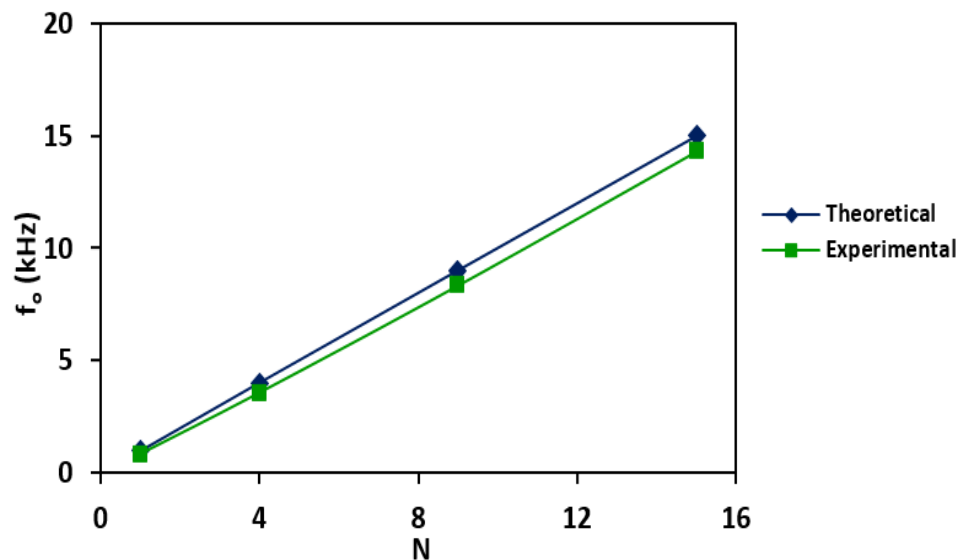
Fig. (12) Graph between Frequency of Oscillations versus Digital Control Word (N)
