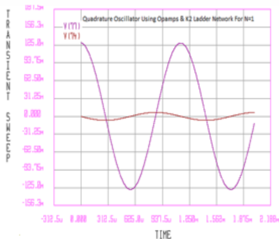
Fig. (8) Output Waveforms of Quadrature Oscillator for Control Word N=1
