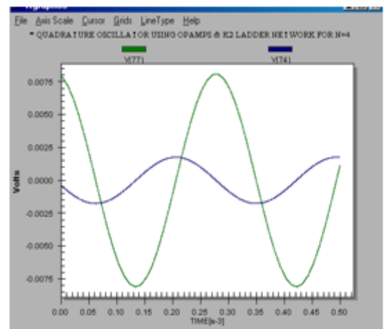
Fig. (9) Output Waveforms of Quadrature Oscillator for Control Word N=4
