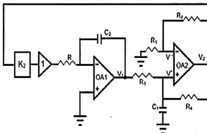
Fig. (7) Digitally Tuned Quadrature Oscillator Circuit
