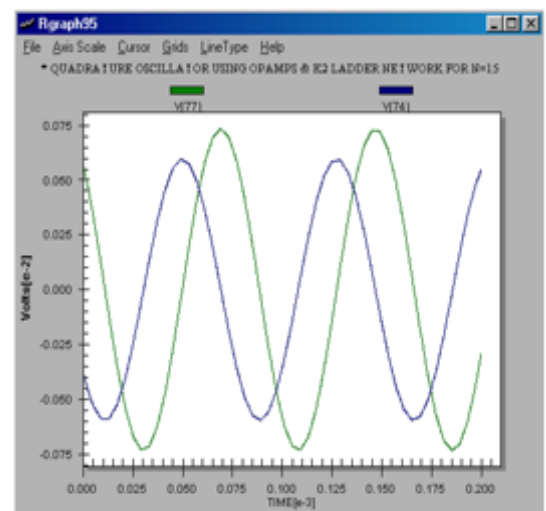
Fig. (11) Output Waveforms of Quadrature Oscillator for Control Word N=15
