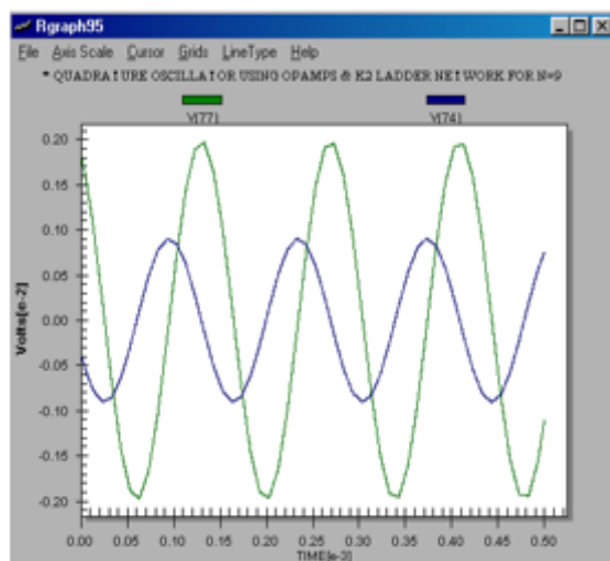
Fig. (10) Output Waveforms of Quadrature Oscillator for Control Word N=9
