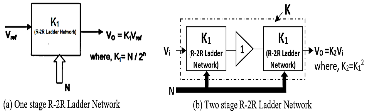
Fig. (4) Block Diagrams of R-2R Ladder Networks
