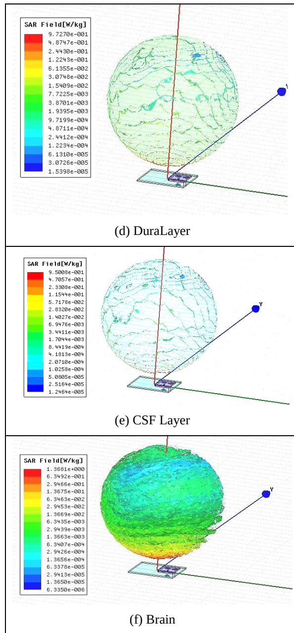
Figure4: SAR values over six layers of phantom model
