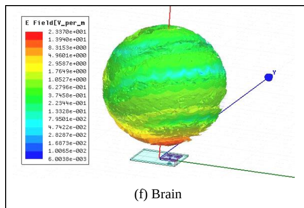
Figure5: E-Field over six layers of phantom model
