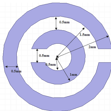
Figure3: Split Ring Resonator (SRR)
