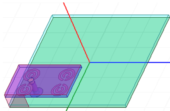
Figure2: PIFA with operating frequency of 3.5GHz
