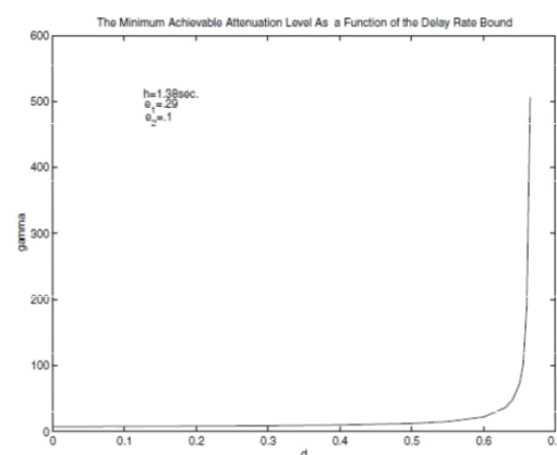
Fig.1: The stabilizability bounds for the time-delay h as a function of d .
