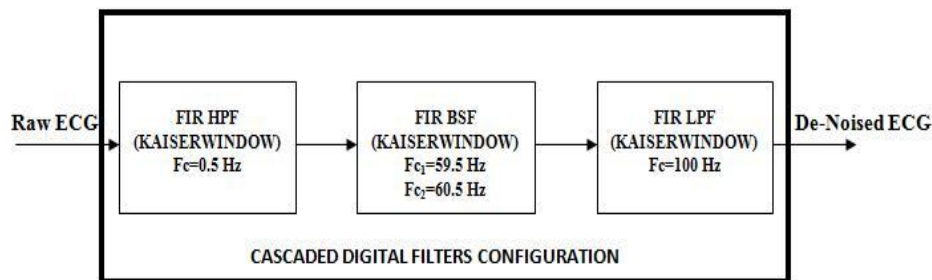
Fig5: Denoising of ECG signal using FIR filter implementation
