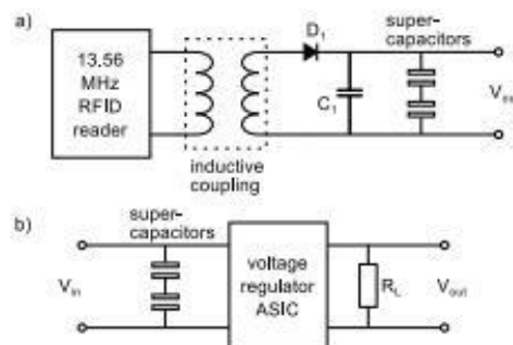
Fig.5 : a) Harvester charging circuit
