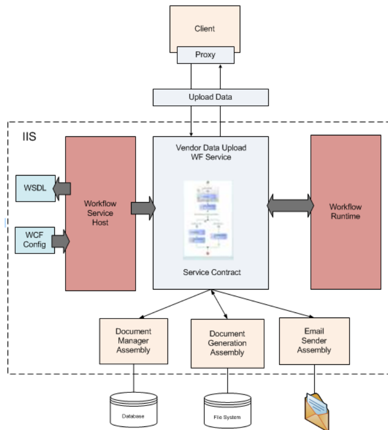
Figure 2: Logical Architecture of Agent Service
