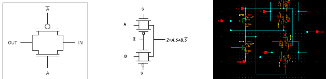
Fig 2.1a: Generalised Transmission Gate, Circuit And Schematic Of Multiplexer.
