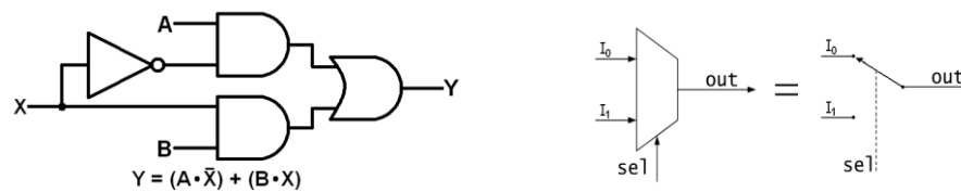
Fig 2a: circuit and symbol of multiplexer.
