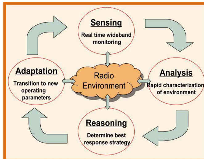
Figure 2: Cognitive cycle [3]
