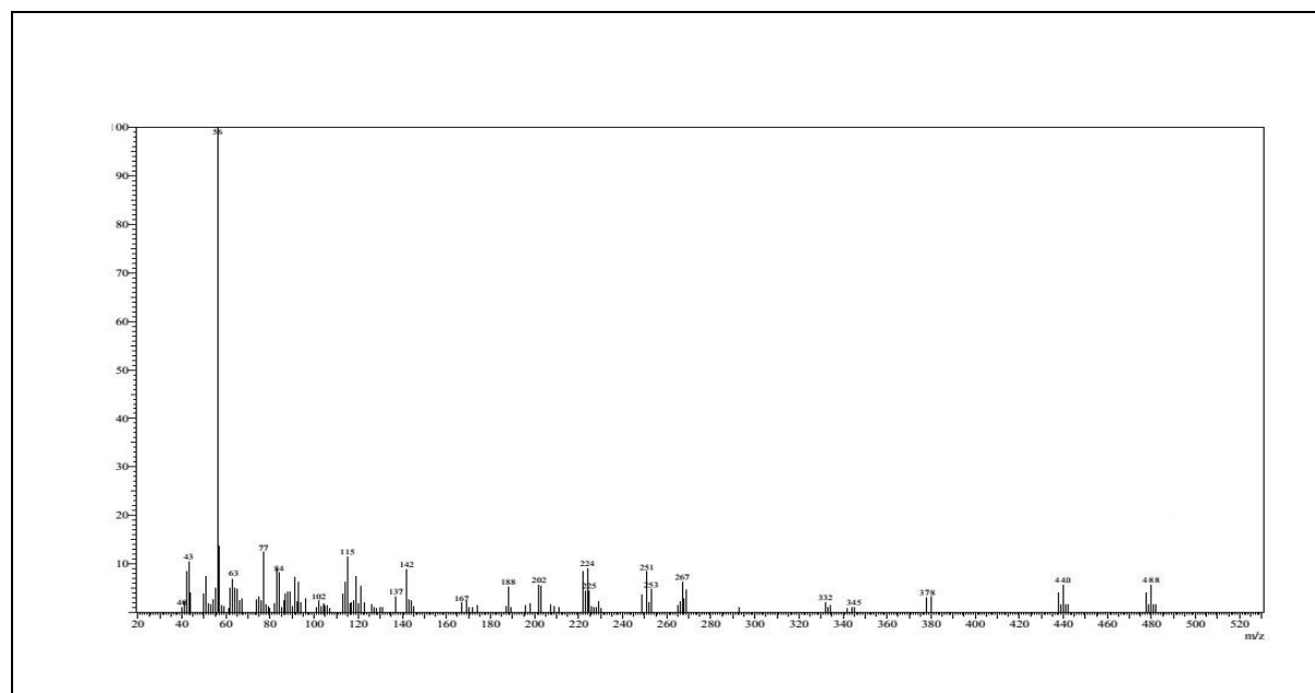
Fig.8 ESI-MASS Spectra of Metal complexes
