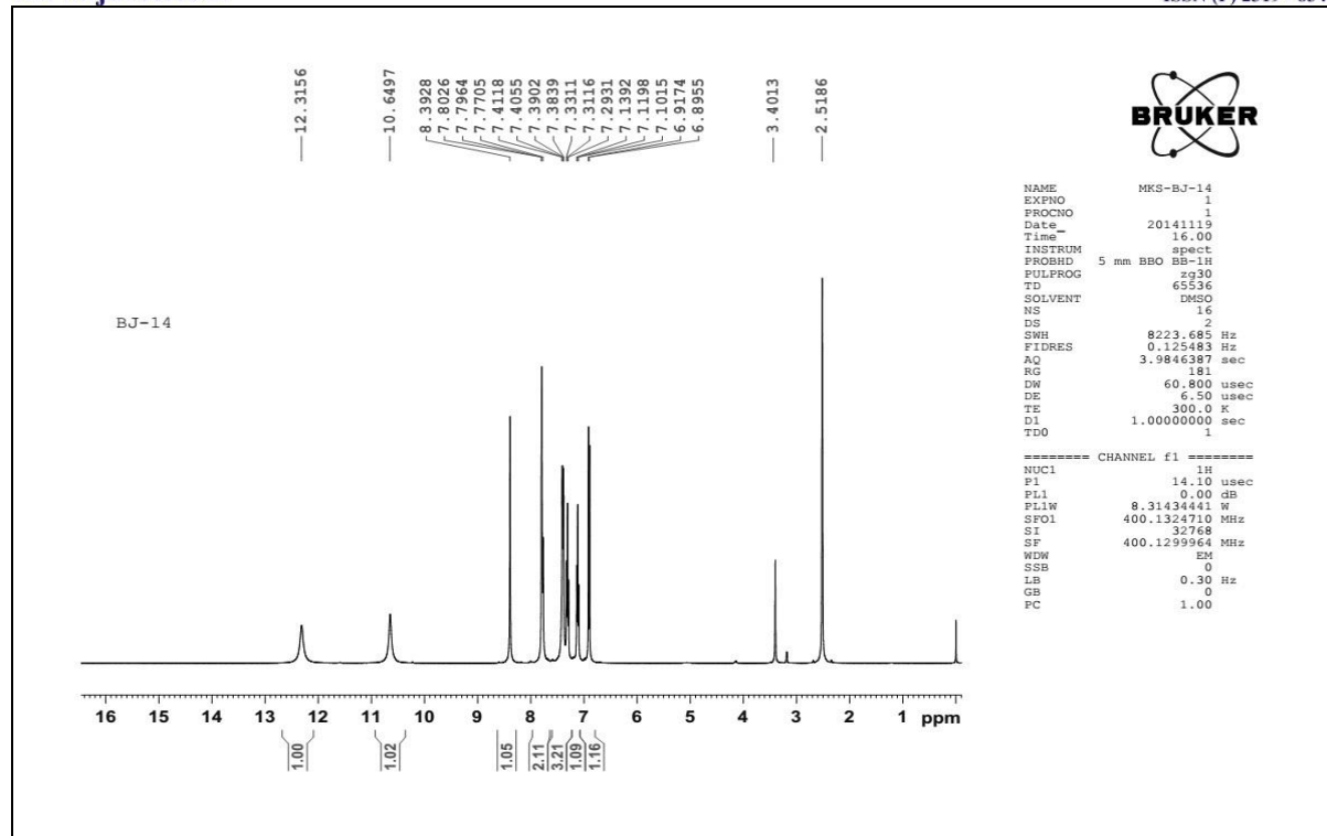
Fig.5 1 H NMR spectra of Ligand
