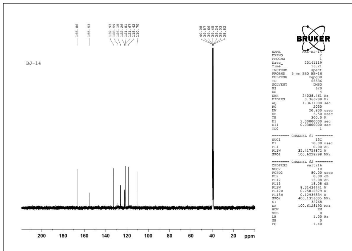
Fig.6 13 C NMR spectra of Ligand
