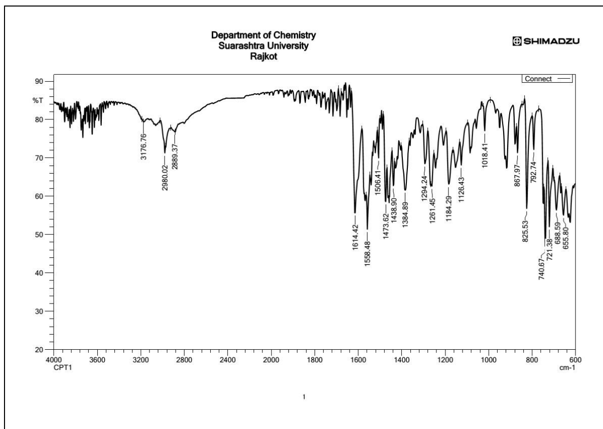
Fig.4 IR Spectra of Ligand
