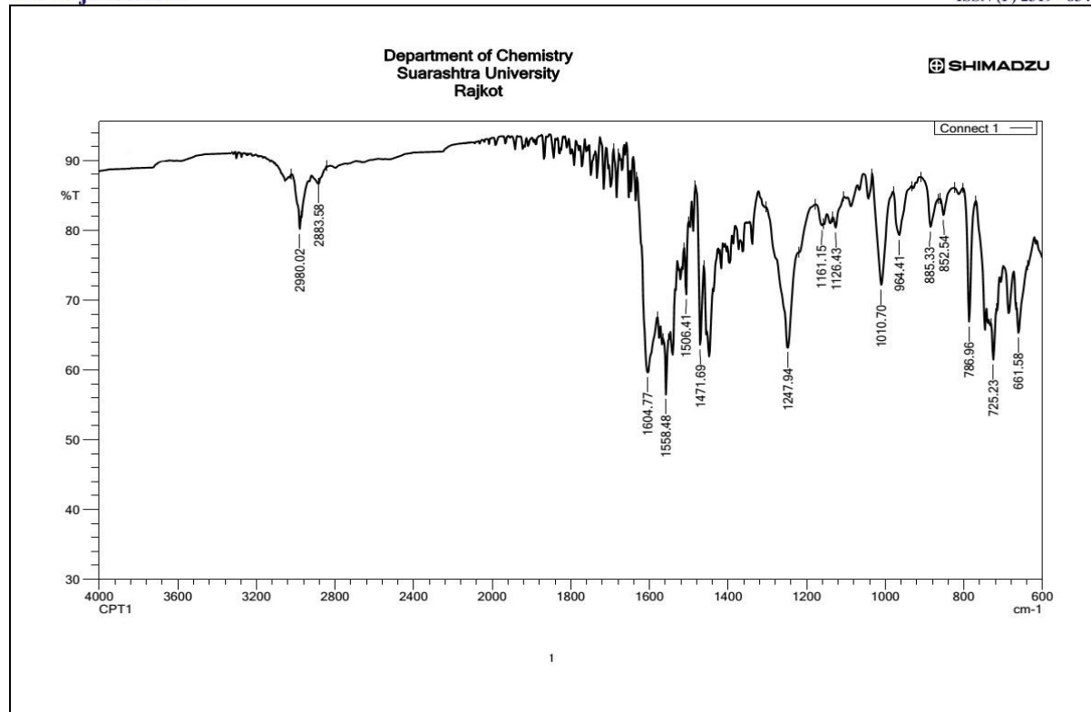
Fig.7 IR spectra of Metal Complex
