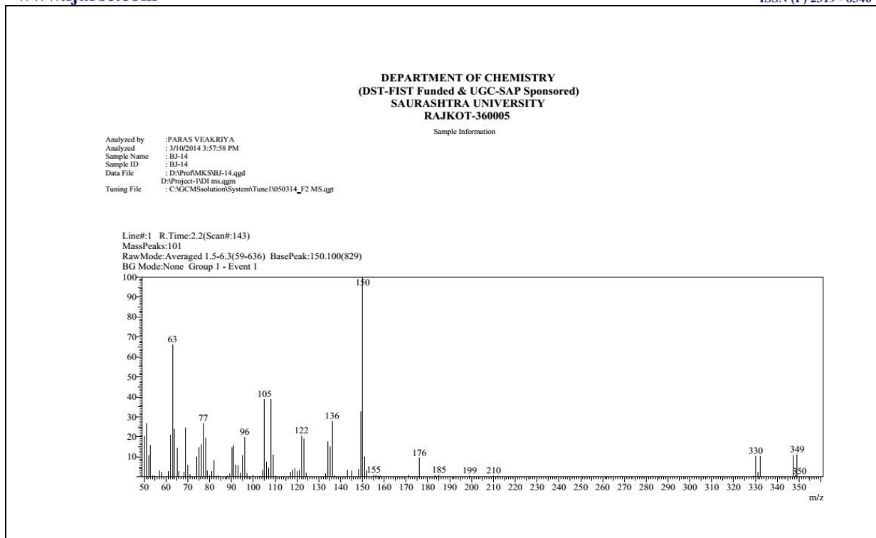
Fig.3 Mass spectrum of ligand BJ-14
