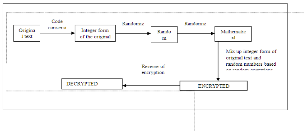
Figure 1. Random secret key generation
