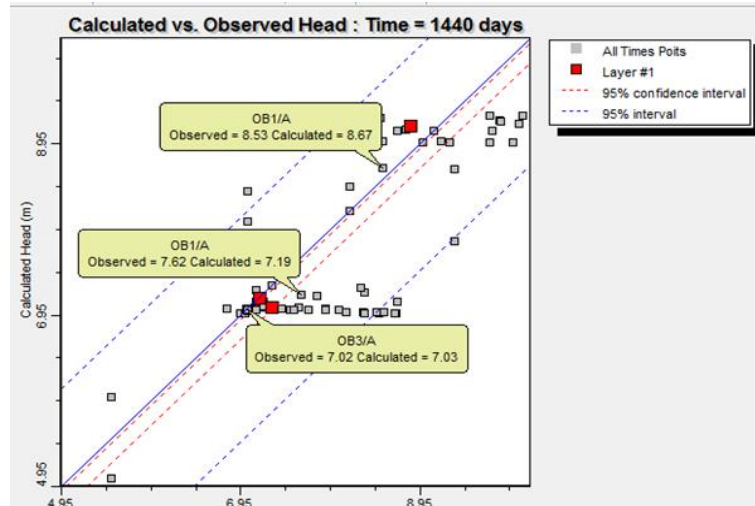
Fig 12: Head Calibration at all time steps
