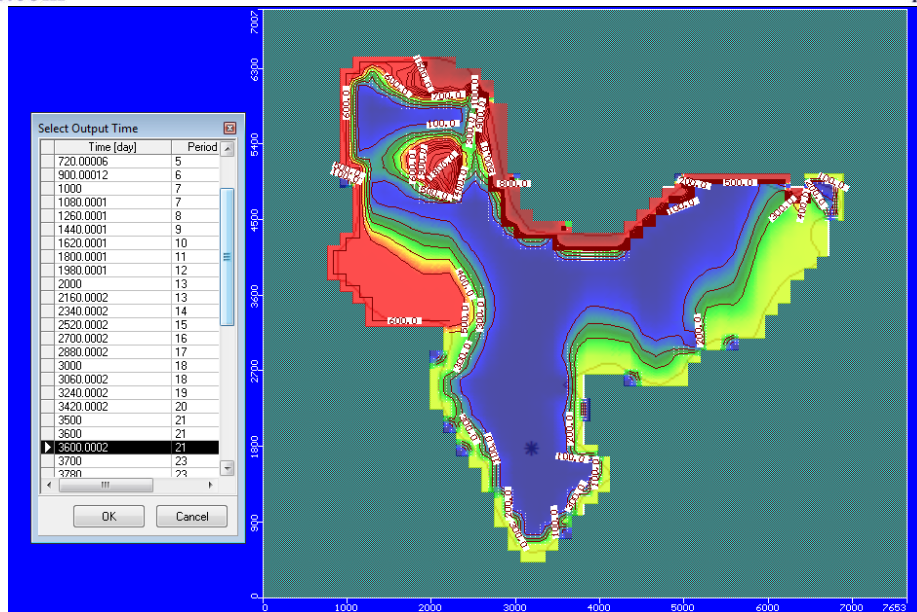
Fig 16: Plume migration at the end of calibration period
