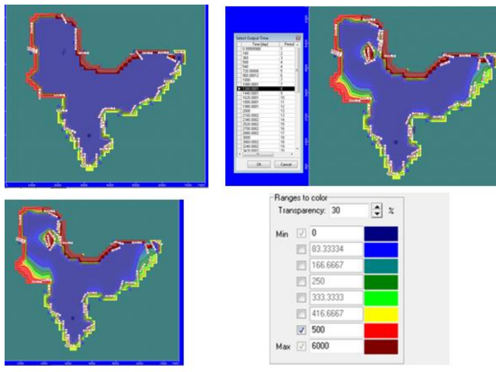
Fig 15: Stages of Plume Migration
