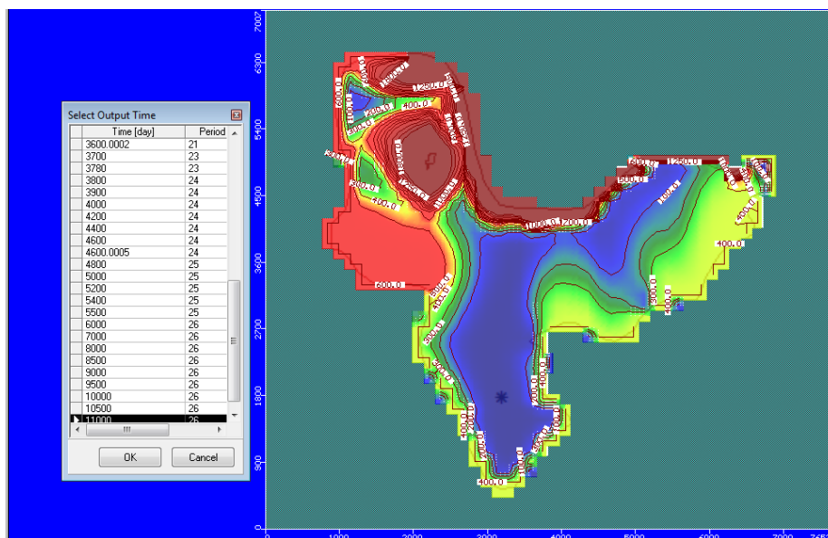
Fig 17: Plume migration at the end of prediction
