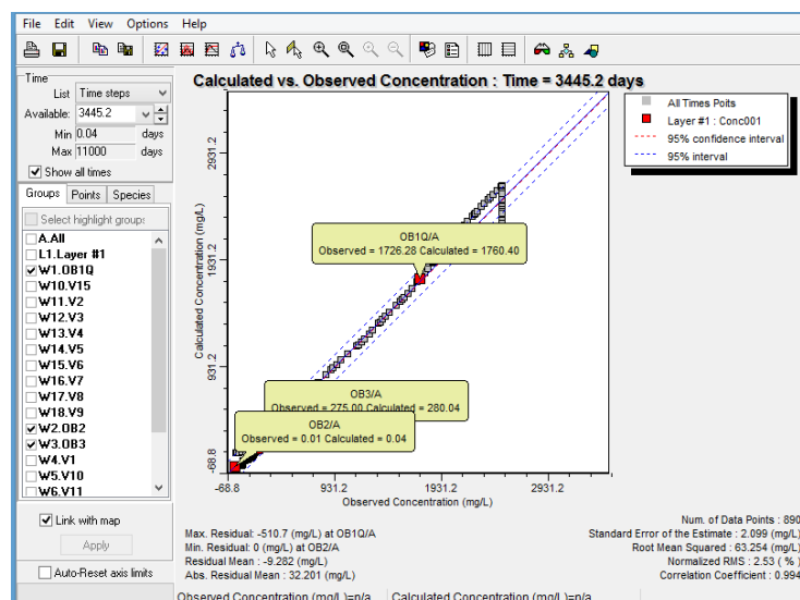
Fig 13: Concentration Calibration at all time steps
