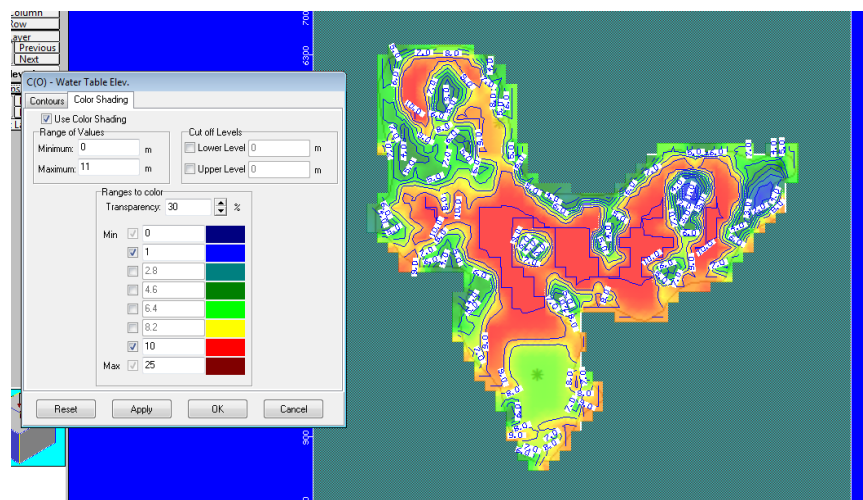
Fig 11 : Water table contour
