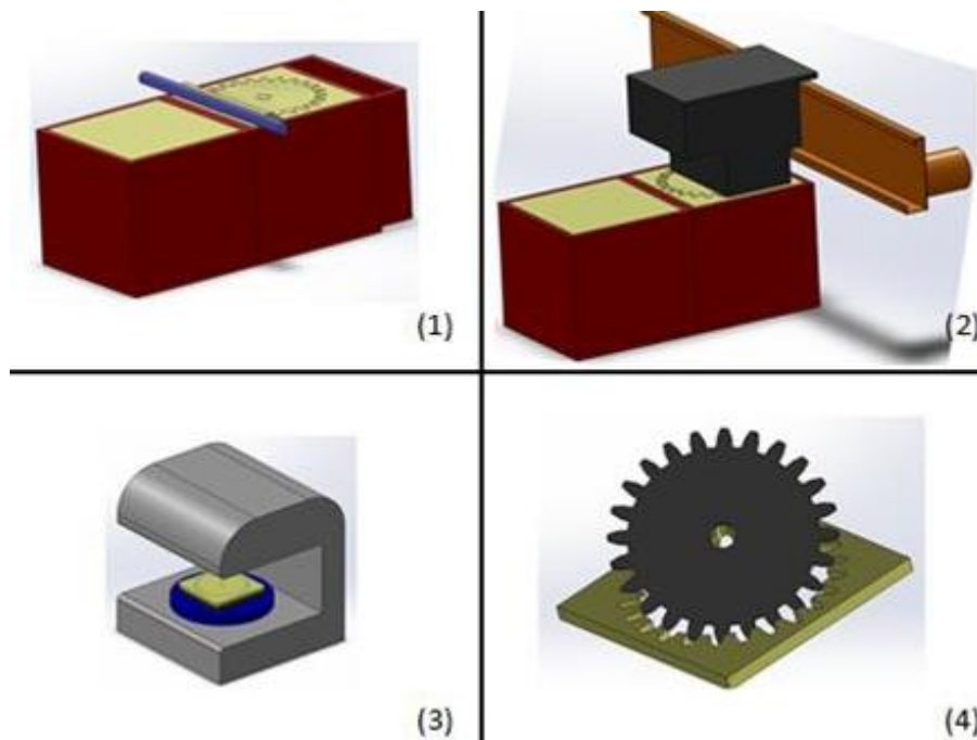
1. Powder pavement; 2. Inhibitor deposition; 3. Sintering in the furnace; 4. Part separation (Fig-2)
