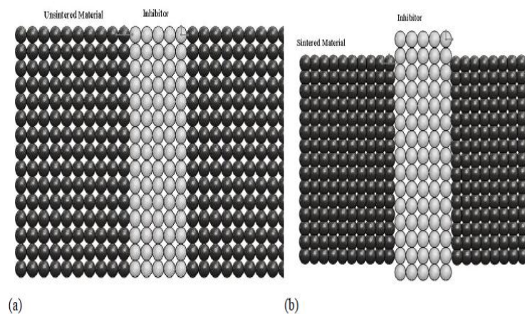
Figure 4 Inhibition Mechanism for SIS-Ceramic (a) Simplified powder distribution before sintering; (b) Shrinkage of building material with inhibitor almost untouched. (The black spheres represent the building material and the white spheres represent the inhibitors)
