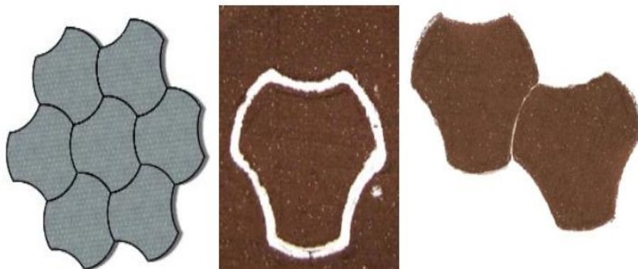
Printed interlocking brick (left) Interlocking pattern for lunar landing pad; (middle) Sintered brick; (right) Printed Bricks Fig-6
