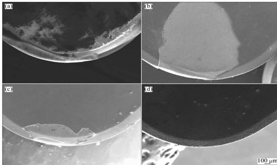
Fig. 8 FE-SEM images of surface morphology of inserts after turning Al-Si alloys: (a) Uncoated insert; (b) NCD coated insert; (c) MCD coated inserts; (d) MCD/NCD coated inserts
