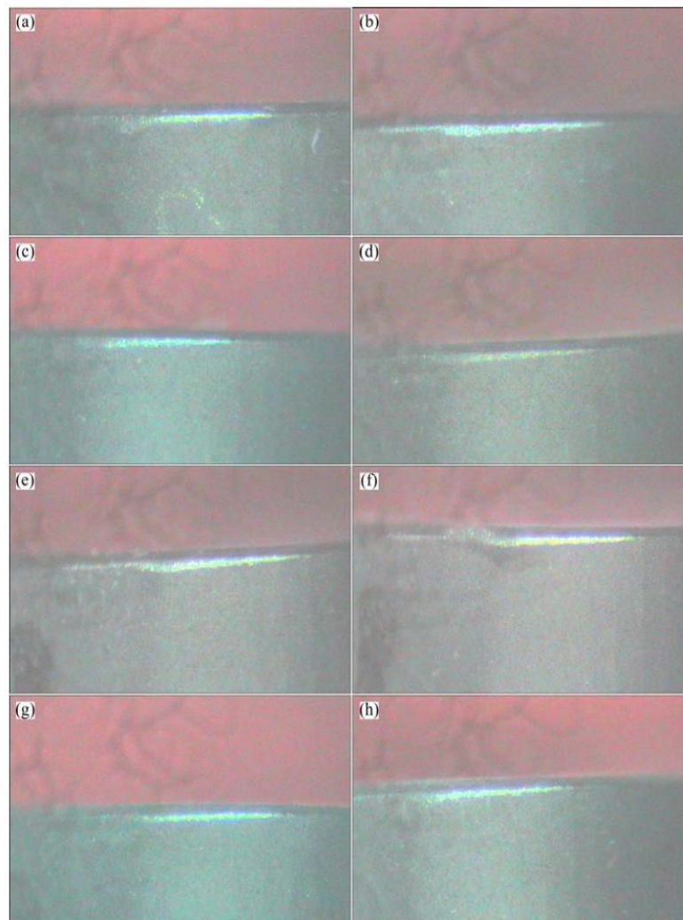
Fig. 7 Images of flank wear of MCD/MCD coated insert after turning 375 m (a), 750 m (b), 1125 m (c), 1500 m (d), 1875 m (e), 2250 m (f), 2650 m (g) and 3000 m (h) of cutting length
