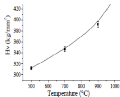
Fig. 3: Variation of the micro-hardness in function of the temperature of annealing.\
