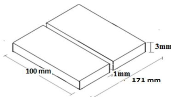
Fig.3.2: Square butt joint for MIG welding
