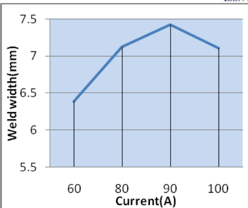
Graph 4.2:Weld Width vs. Current
