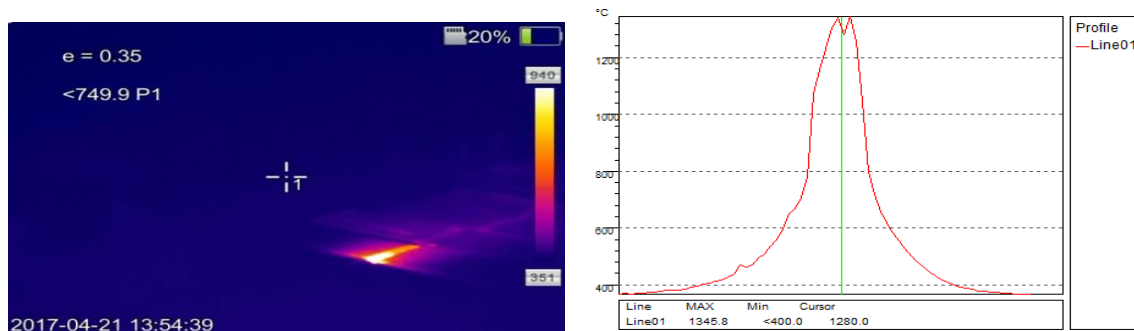
Fig 4.1: Temperature profile at current 60 ampere
