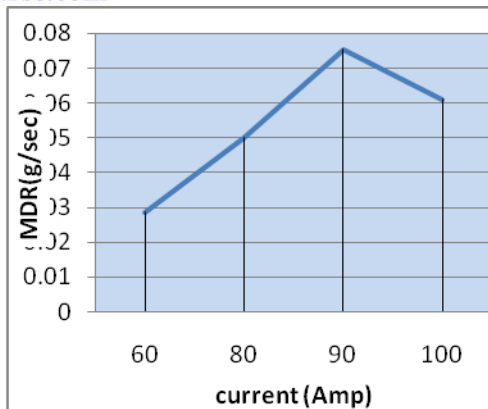
Graph 4.1:MDRvs. Current
