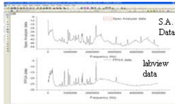
Figure 11 : Comparison of FFT by FPGA (or LabVIEW) and FFT by Agilent N1996A
