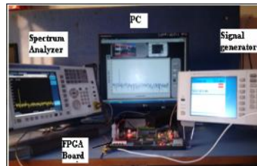
Figure 12 : Experimental Set-Up for Spectrogram
