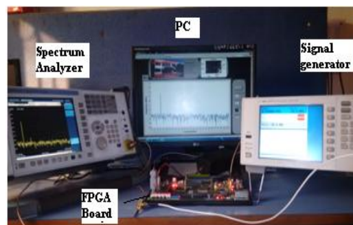
Figure 10 : Single channel Spectroscopy experimental setup
