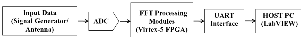
Figure 1 : Block diagram of System
