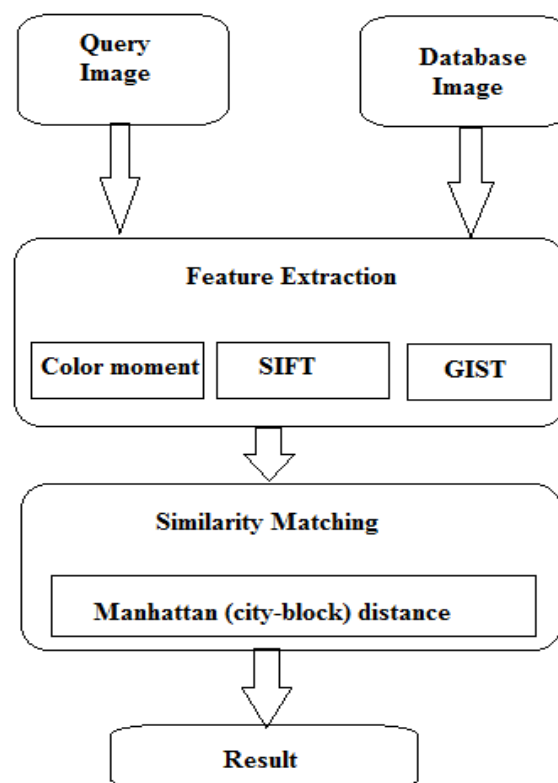
Fig. 2. Architecture of CBIR for Remote sensing images
