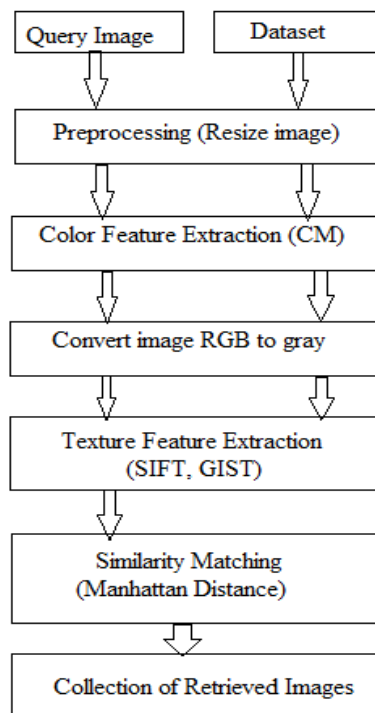
Fig. 5. Flowchart for CBIR System.
