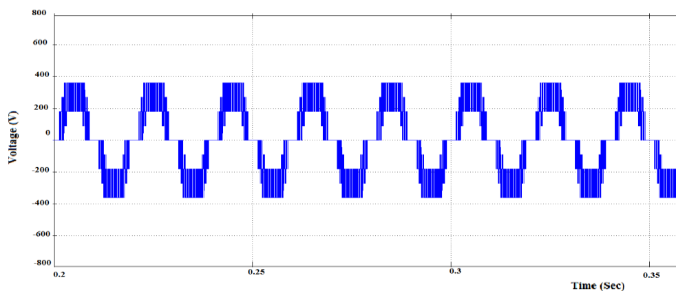
Fig: 4. Output Voltage with HBZ-S Inverter
