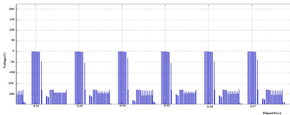
Fig: 5. Reduced Voltage stress on Capacitors
