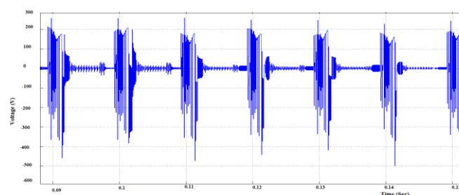
Fig: 3 Output Voltage without HBZ-S Inverter
