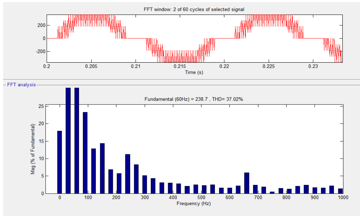
Fig 7. FFT Analysis with HBZ-SI
