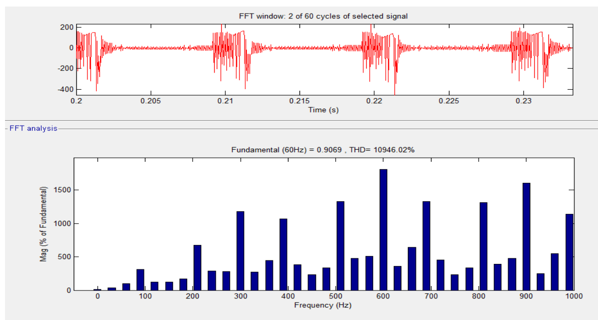
Fig 6. FFT Analysis without HBZ-SI
