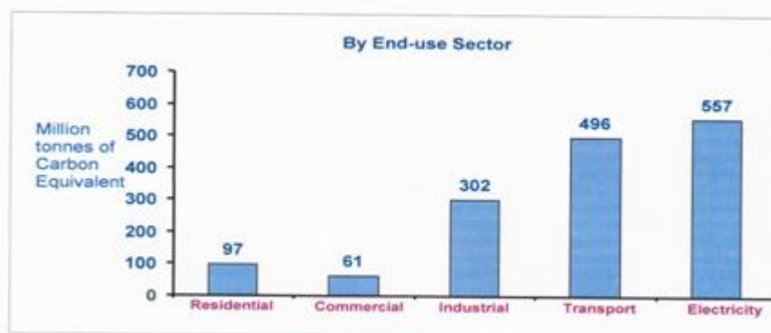
Figure-1: Sector wise world CO 2 emissions
