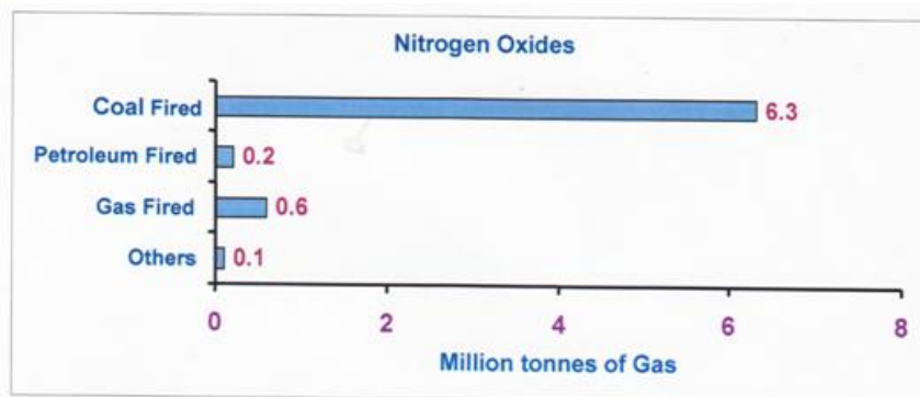
Figure-5: World NO x emissions from electricity generation in 1999
