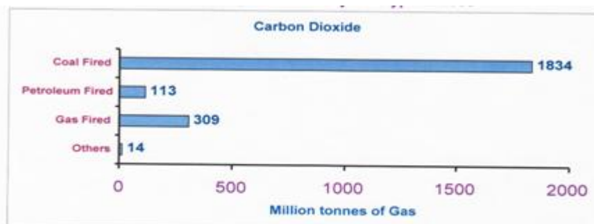
Figure-3: World CO 2 emissions from electricity generation in 1999
