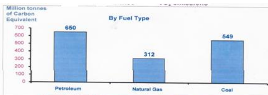
Figure-2: World CO 2 emissions by fuel type in 1999
