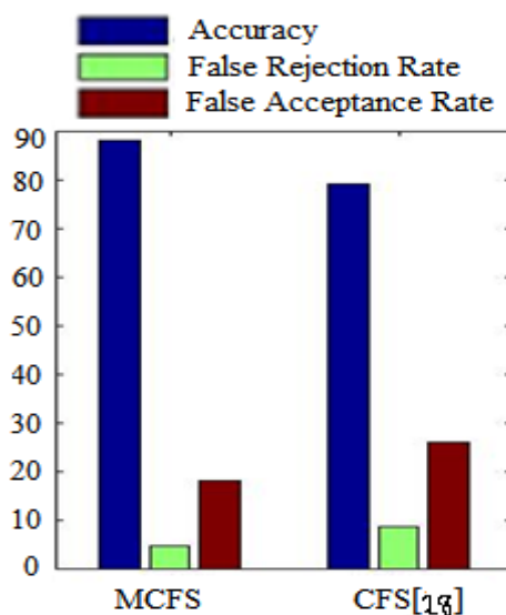
Fig.3 : Segmentation performance of the proposed against existing system [28]
