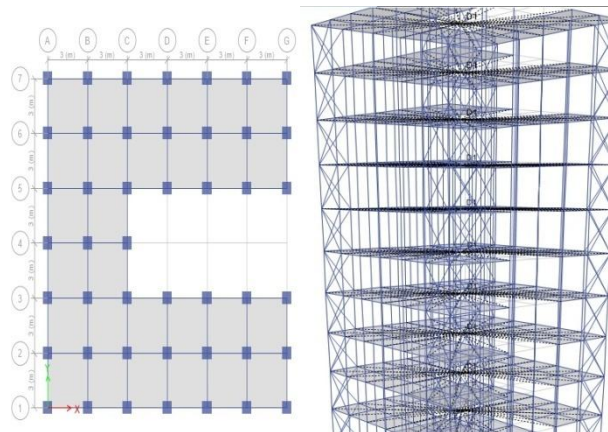
Fig. 1. a) Plan of Moment Resisting Frame C-Section building
