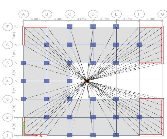
c) Plan of shear wall system
