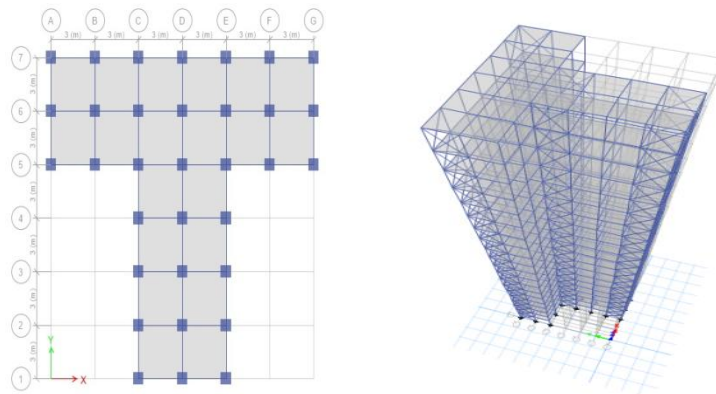
Fig. 1. a)Plan of Moment Resisting Frame C-Section building
