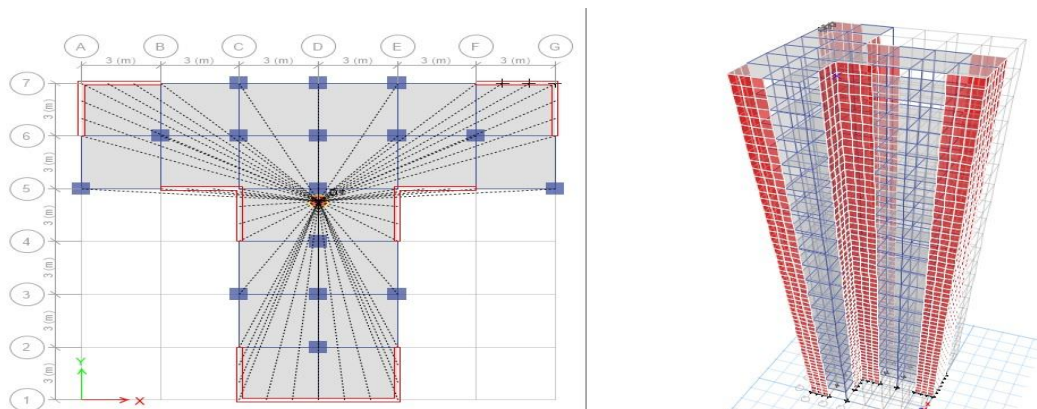
c) Plan of shear wall system
