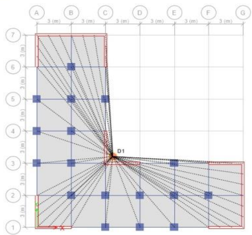
c) Plan of shear wall system
