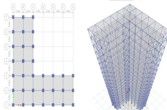
b)Plan of Braced frame system
