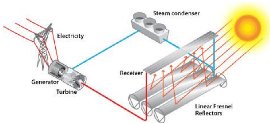
“Fig”.2: Linear Frensel Power Plant
