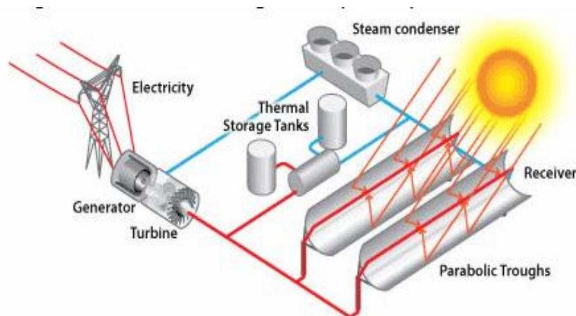
“Fig”.1 Parabolic trough
