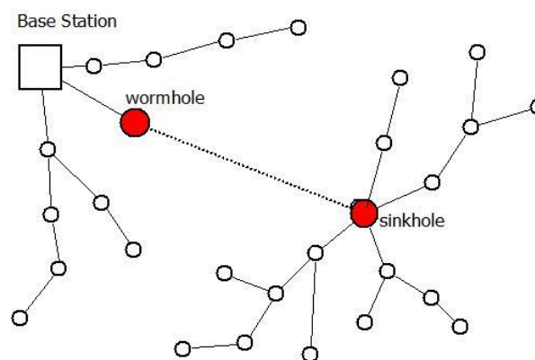
Fig. 7: A laptop class adversary utilizing a wormhole to make a sinkhole
