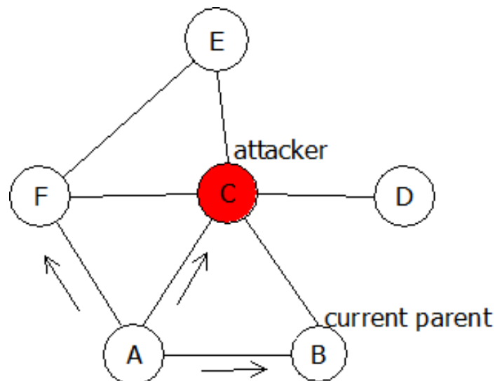
Fig. 1: Node C gets the "route update packet" of node A
