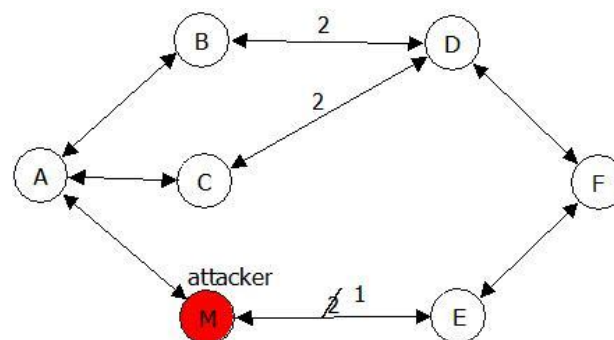
Fig. 6: Sinkhole attack in Tiny AODV protocol
