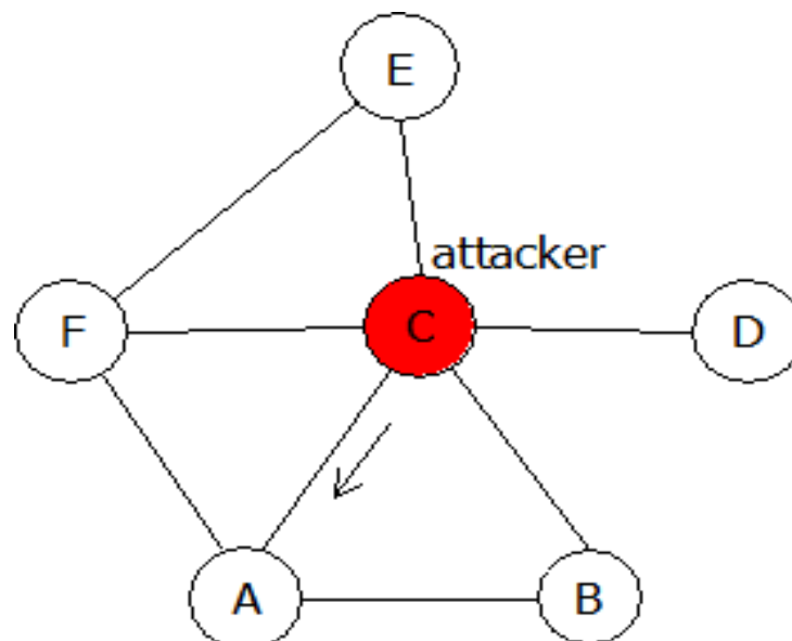
Fig. 2: Node C sends a malicious packet to node A imitating as node B
