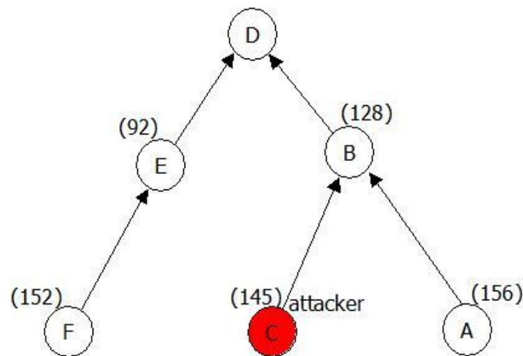
Fig. 3: Multi hop LQI routing protocol
