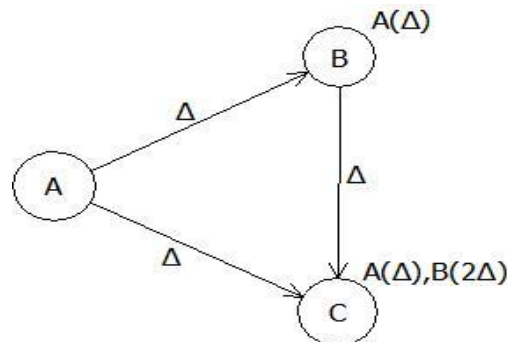
Fig. 8: Gradient setup in directed diffusion routing protocol
