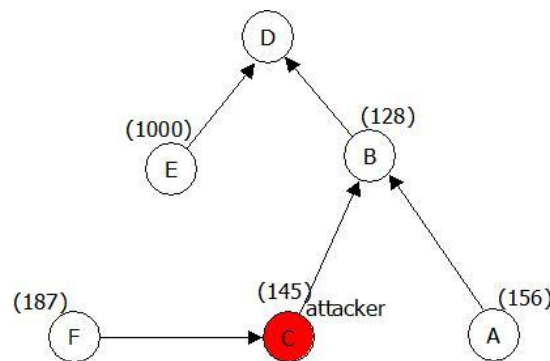
Fig. 5: Way 2 of attack
