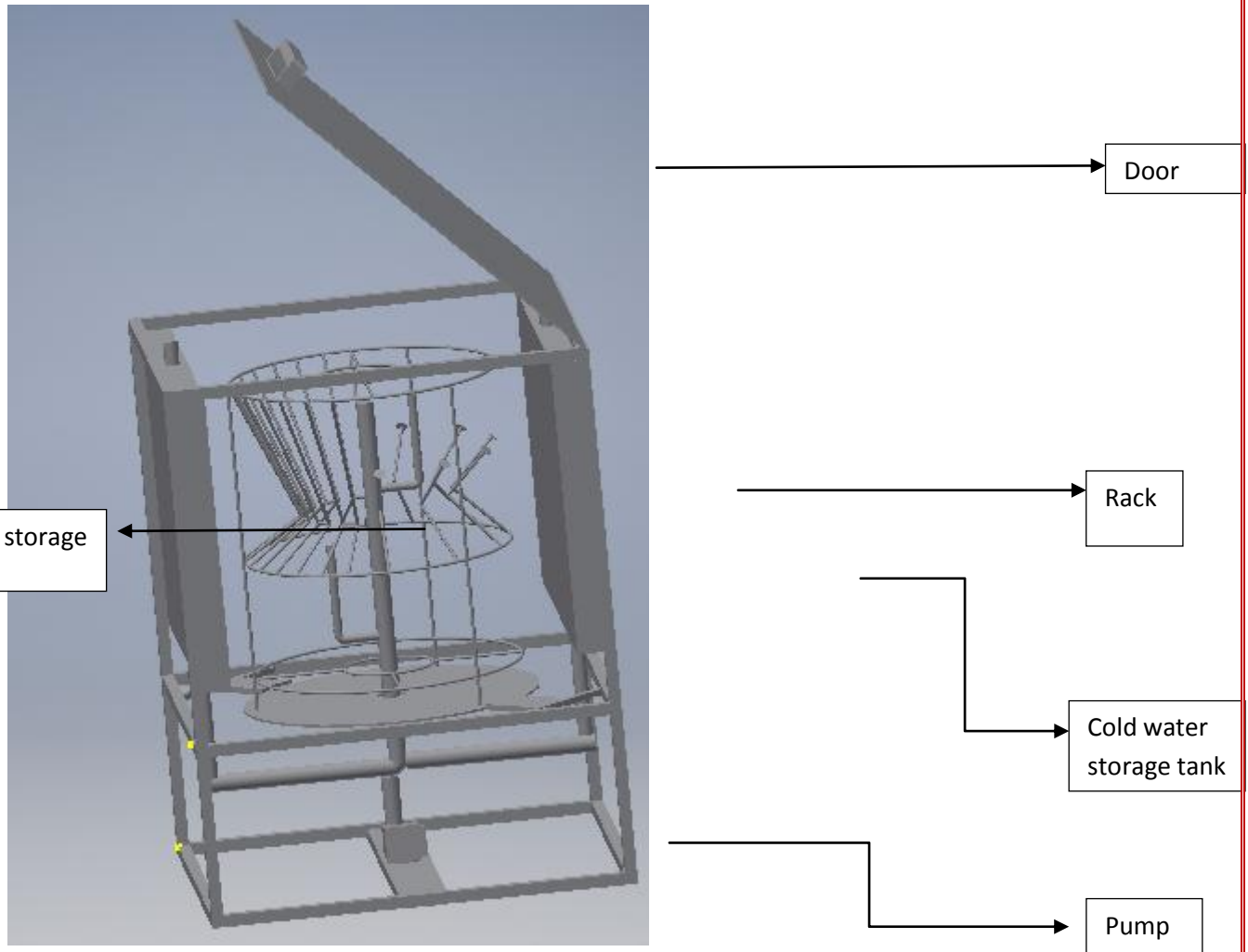
Fig.6.1 CAD model of set up
