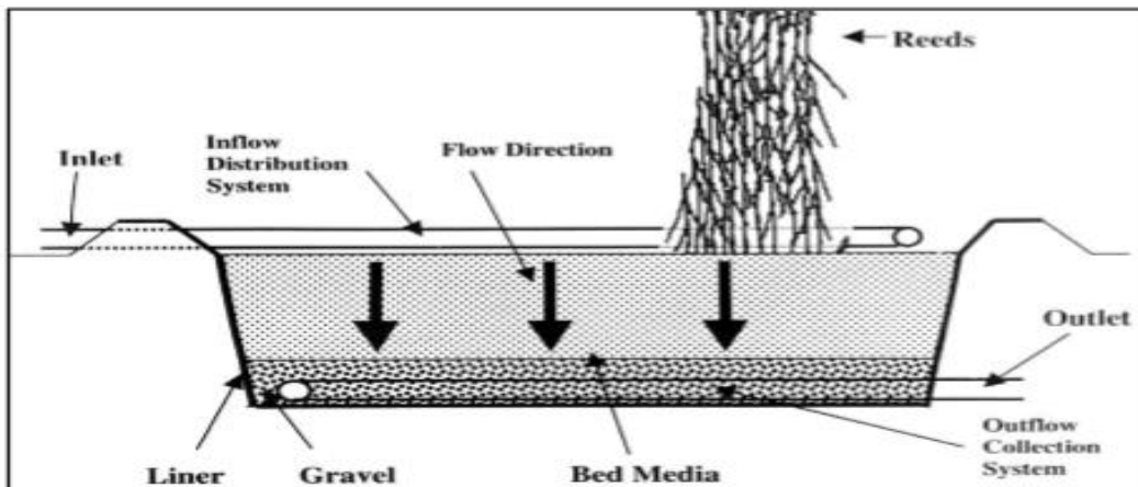
Fig. 2 : Vertical (flow system) root zone filter
