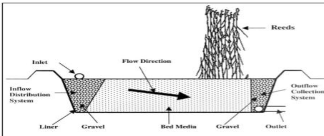
Fig. 1 : Horizontal (flow system) root zone filter
