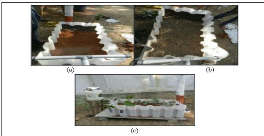
Fig. 5 : Construction of pilot scale RZT reactor a) soil layer b) compost layer c) final set up after plantation
