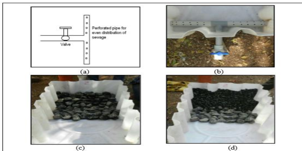
Fig. 4 : Development of Root Zone Treatment (RTZ) system reactor: a) distribution pipe at top (inlet) b) underdrainage pipe at bottom (outlet) c) constructional details d) constructional details
