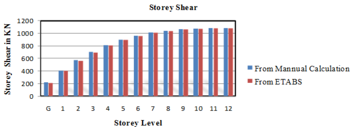
Fig. 2 Graphical Representation Of Storey Shear From ETABS And Manual Calculation
