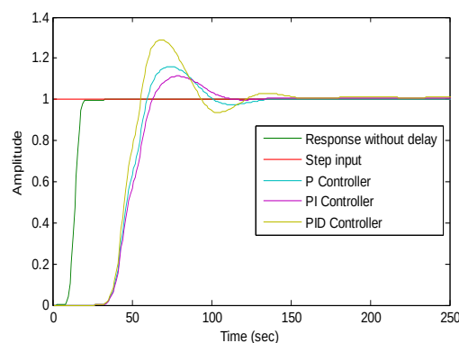
Fig. 14: Step response of conventional controllers
