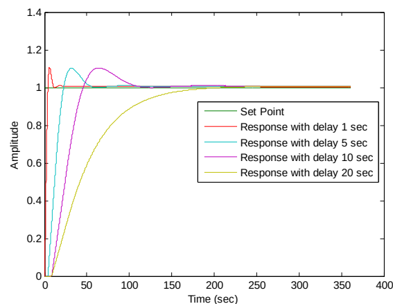
Fig. 4: Step response of PI controller with various delays
