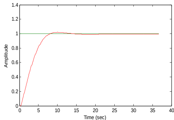
Fig. 7: Response of neural network controller
