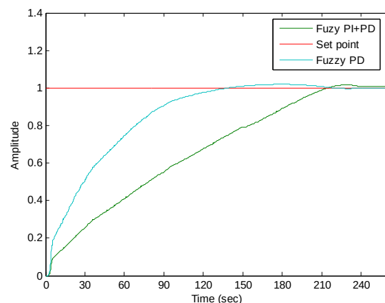
Fig. 16: Comparison the response of fuzzy PD and PI+PD controllers
