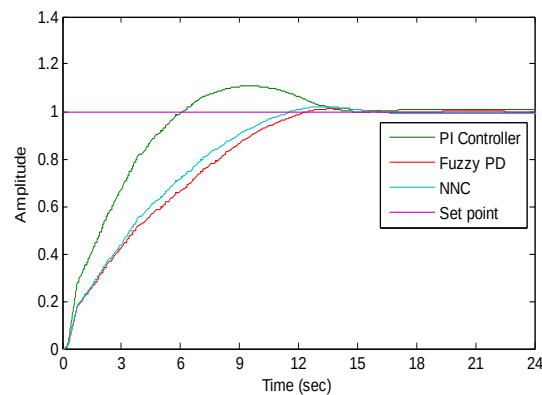
Fig. 11: Comparison of different controllers
