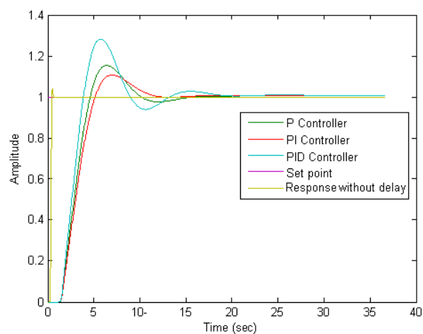
Fig. 3: Step response of conventional controllers
