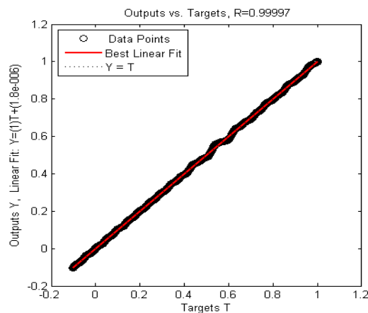
Fig. 9: Linear regression graph between network output and targets
