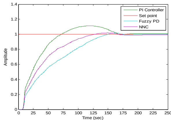
Fig. 18: Comparison of various controllers
