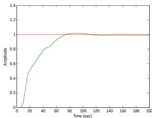
Fig. 17: Response of neural network controllers
