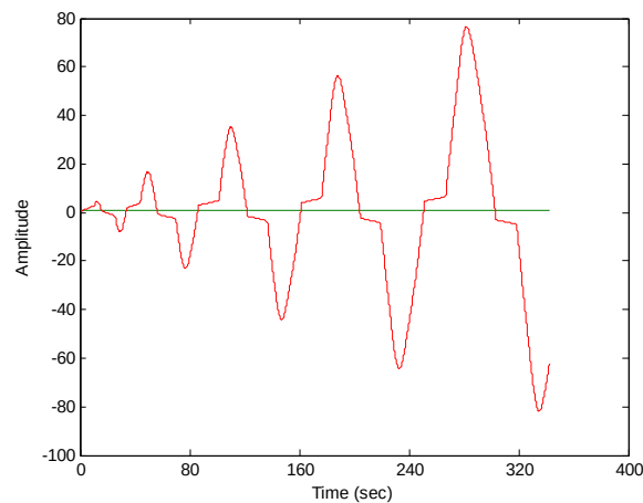
Fig. 5: Step response of Fuzzy PI controller
