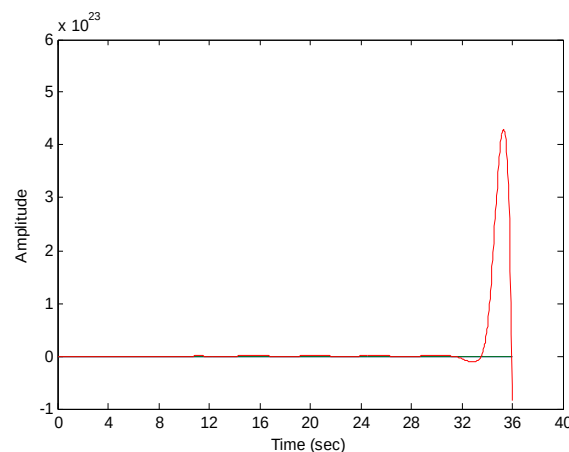
Fig 2: Step response of uncontrolled process
