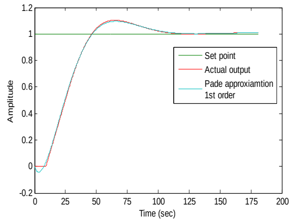
Fig. 12: Padé first order approximation
