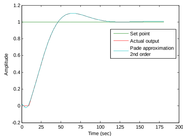
Fig. 13: Padé second order approximation
