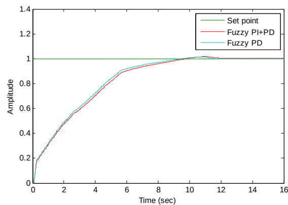
Fig. 6: Step response of Fuzzy PD and PI+PD controller
