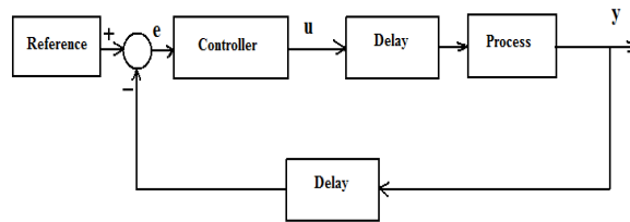
Fig. 1 Example of time delay system
