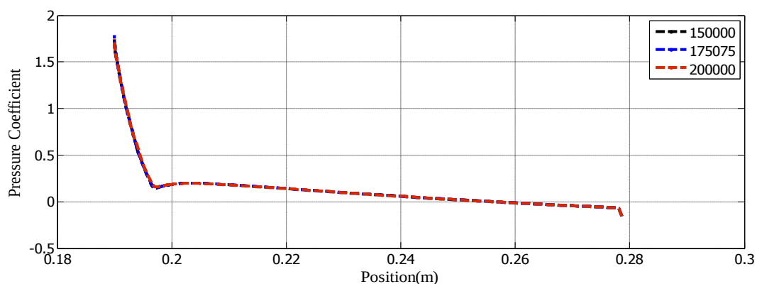
Fig. 1: Variation of Pressure coefficient with upper body of a blunted tangent ogive ( r/R = 0.4 , and p = 250\text{mm} ) for various grids showing grid sensitivity.
