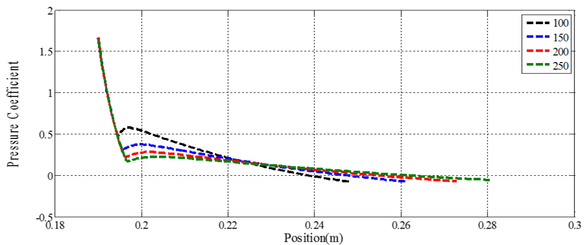
Fig. 4: Variation of pressure coefficient with upper body of a blunted tangent ogive at (a) r/R = 0.4 ( r = 10 mm, R = 25 mm) for (a)100mm (b)150mm (c)200mm (d)250mm
