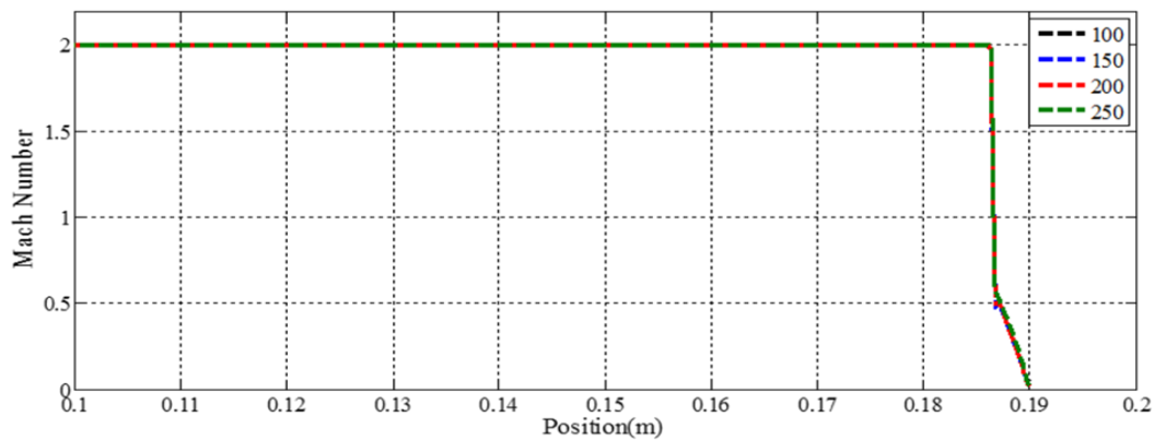
Fig. 2: Variation of Mach number with position along the axis of a blunted tangent ogive at r/R = 0.4 ( r = 10 mm, R = 25 mm) for (a)100mm (b)150mm (c)200mm (d)250mm
