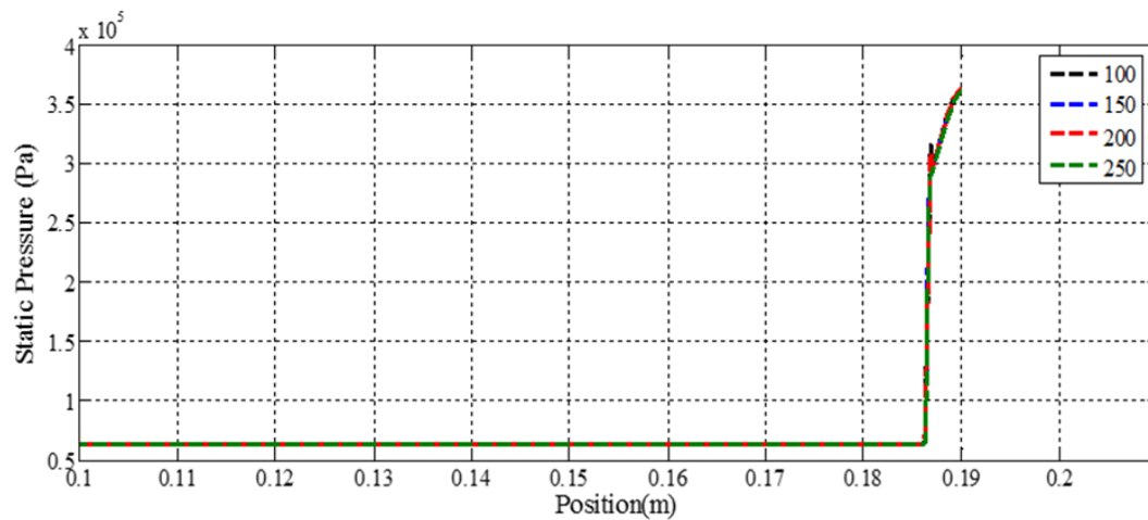
Fig. 3: Variation of Static Pressure with position along the axis of a blunted tangent ogive at r/R = 0.4 ( r = 10 mm, R = 25 mm) for (a)100mm (b)150mm (c)200mm (d)250mm
