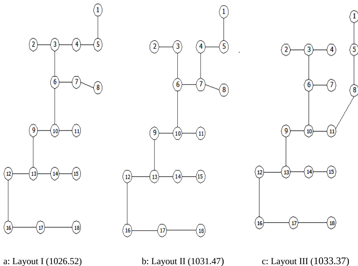
Fig. 2: Three most competitive layouts for the 18-node sewerage system
