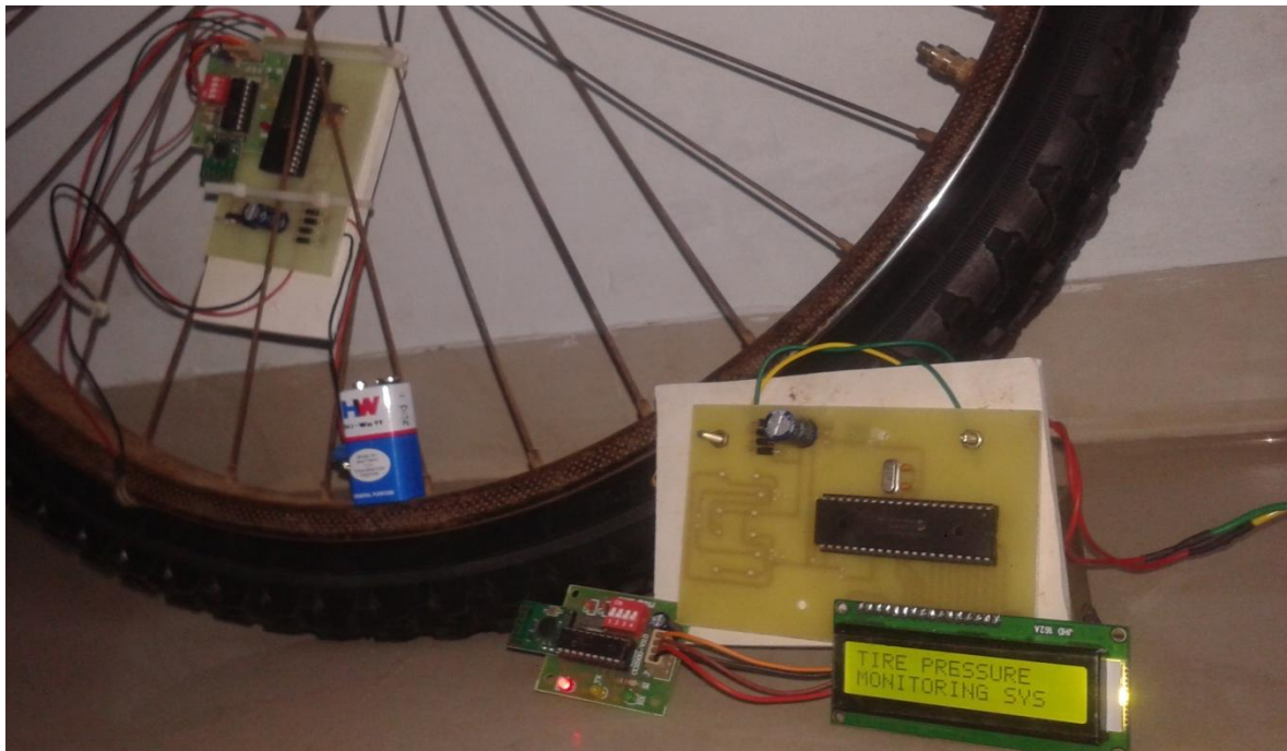
Figure 4.The Tyre Pressure Monitoring System Performance Analysis
