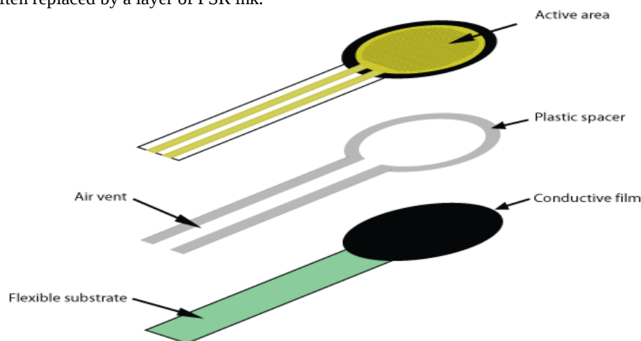
Figure 2.1. Force Pressure Sensor
