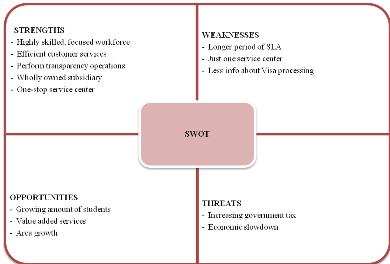
Figure 4: SWOT Analysis
