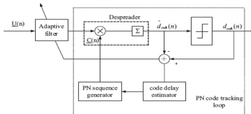
Fig.1. The conventional coherent receiver - joint detection and PN code tracking.
