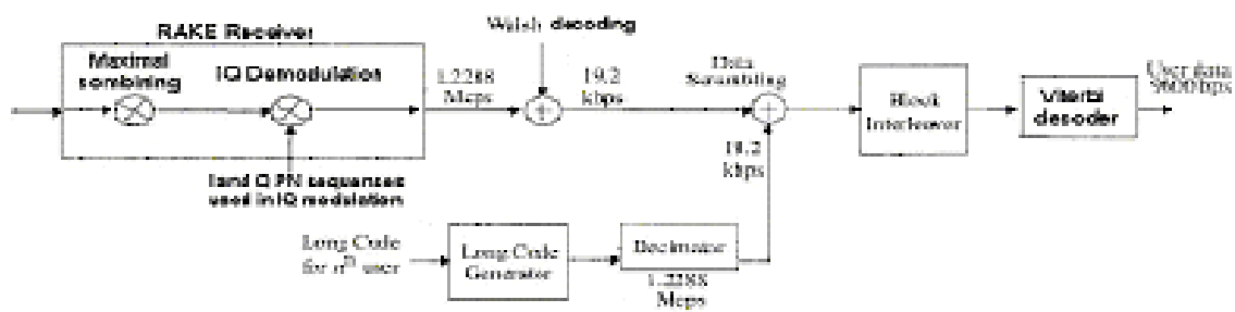
Fig: 7 CDMA Receiver Demodulation Process.
