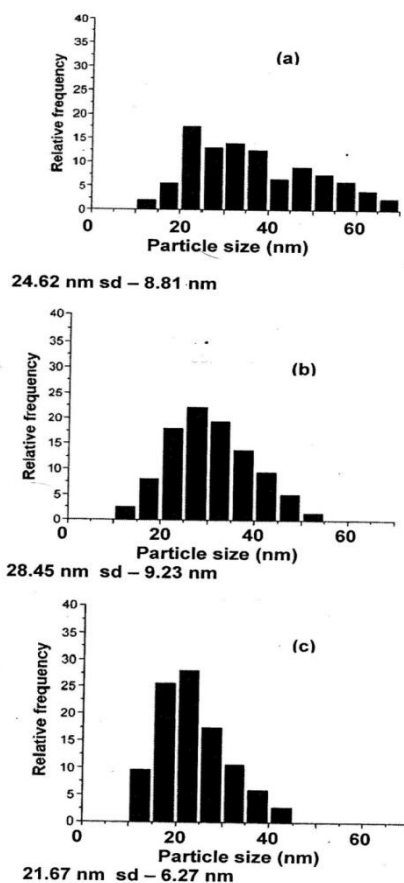
Fig.4 – Particle size distribution of coated ZnO NPs (a) 10^{-4} \text{ M Zn}^{2+}
