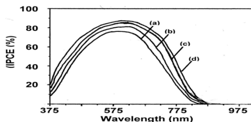
Fig.2 – IPCE versus wavelength of bare \text{TiO}_2 and ZnO coated \text{TiO}_2 DSSC (b) bare \text{TiO}_2
