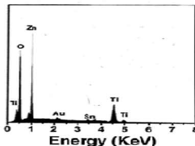
Fig.1 – EDAX spectrum of ZnO coated \text{TiO}_2 coated DSSC( 10^{-5} \text{Zn}^{2+} )
