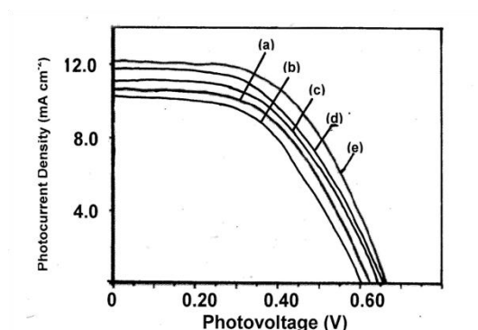
Fig.3 – Photocurrent – photovoltage characteristics of bare \text{TiO}_2 and ZnO coated \text{TiO}_2
