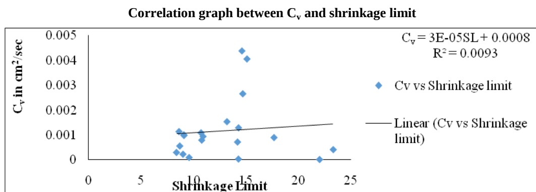
Fig 6 Correlation graph between C_v and shrinkage limit
