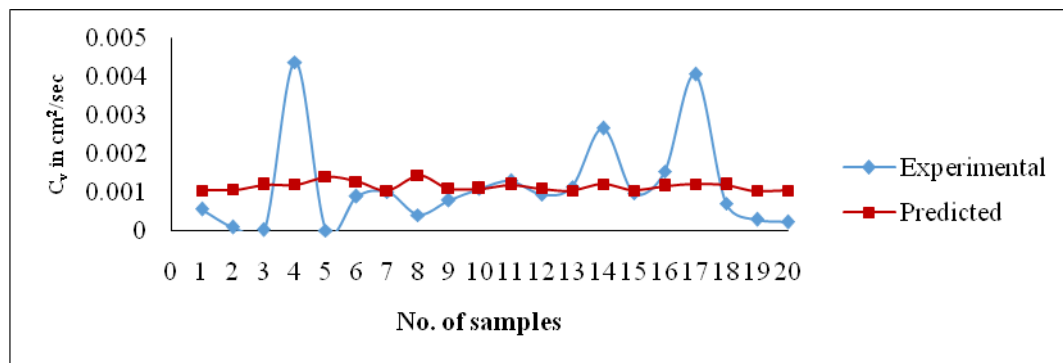
Fig 7 Comparison between experimental and predicted C_v value for shrinkage limit
