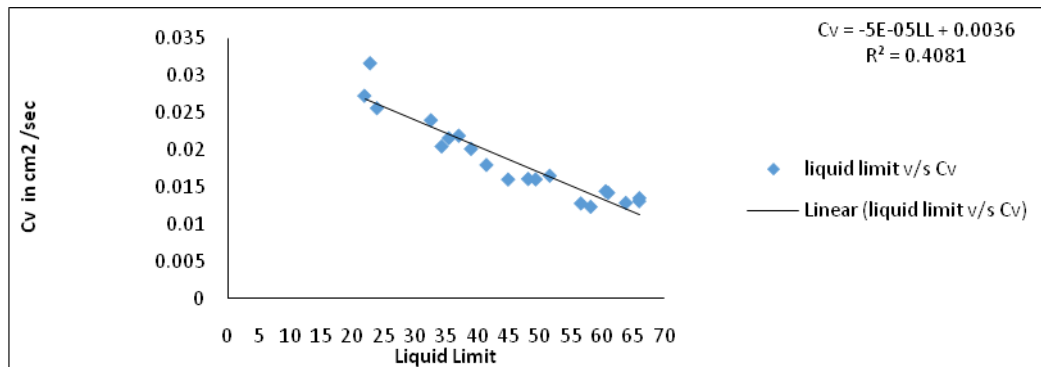
Fig 2 Correlation graph between C_v and liquid limit
