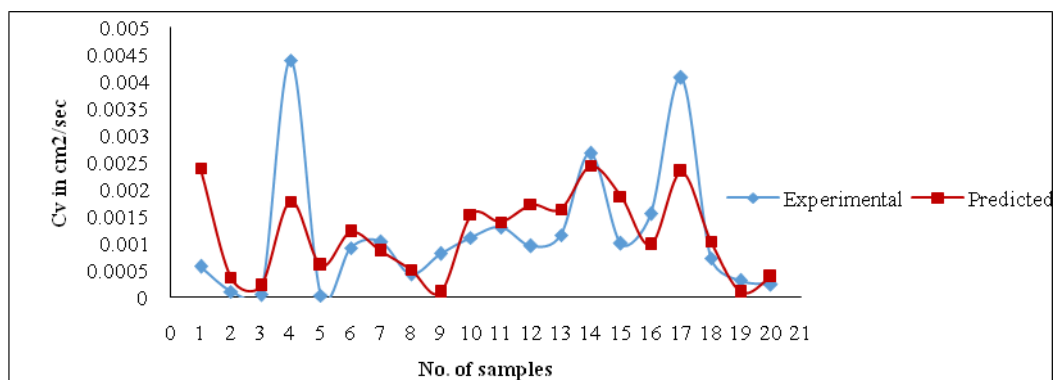
Fig 3 Comparison between experimental and predicted C_v value for liquid limit
