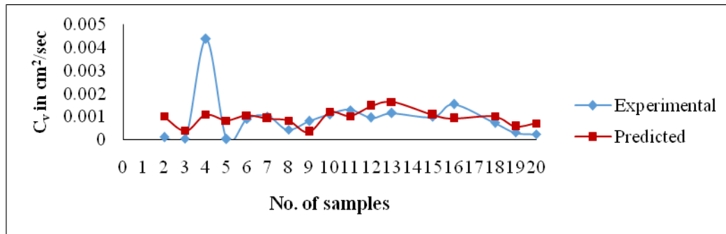
Fig 5 Comparison between experimental and predicted C_v value for plastic limit
